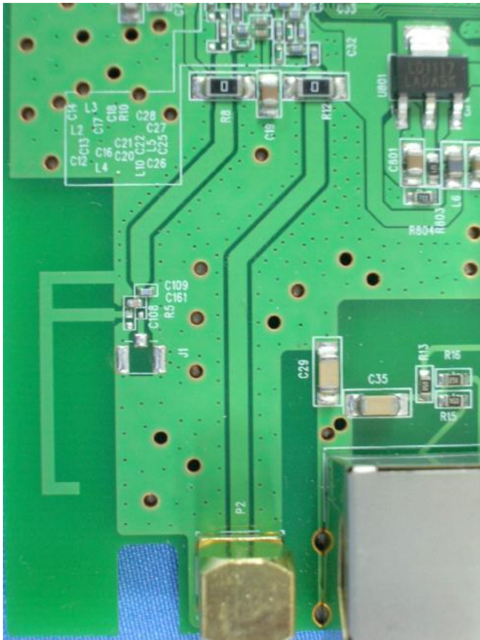
(11) EUT Photo
