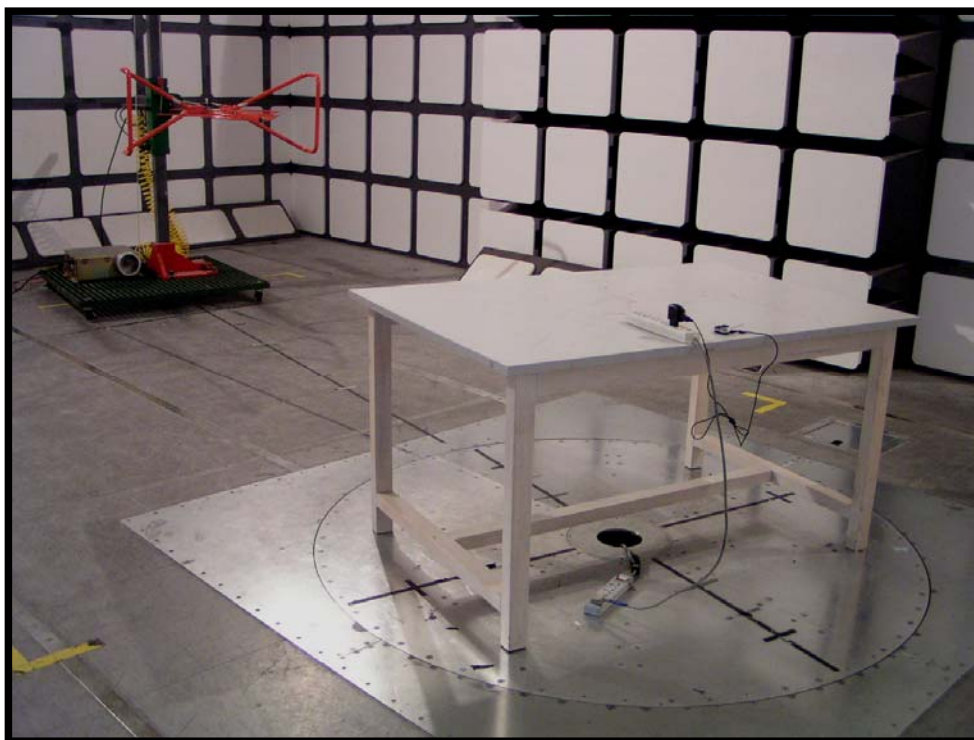
Radiated Emissions - Rear View (Below 1GHz) for charging mode
