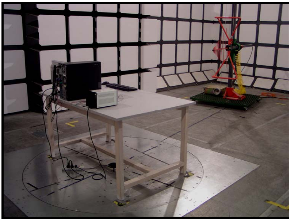
Radiated Emissions - Rear View (30-1000MHz) for transmitting mode
