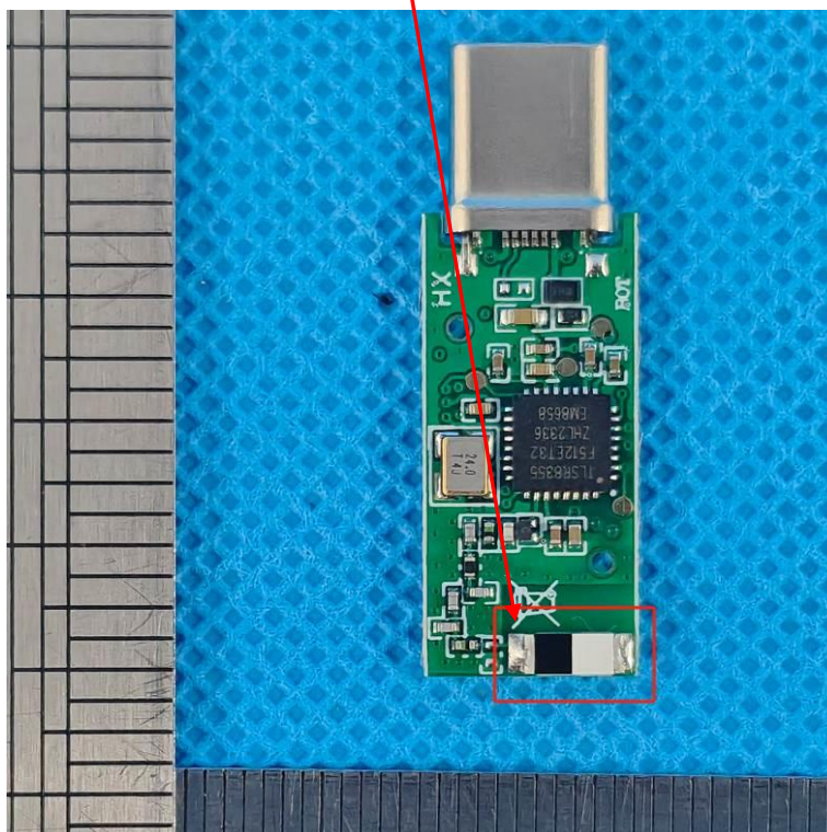
View of wireless antenna
