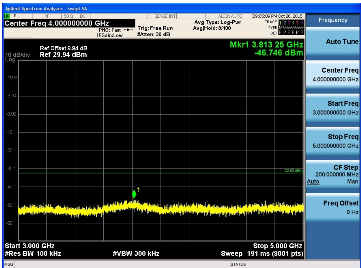
(Plot 4.6.2 C3: Channel 11: 2462MHz @ 802.11g)
