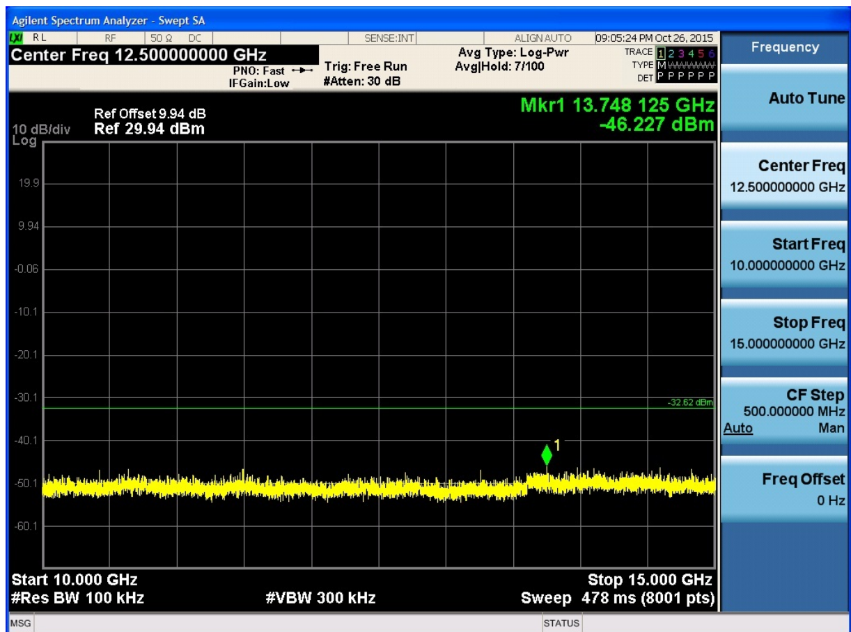
(Plot 4.6.2 C5: Channel 11: 2462MHz @ 802.11g)
