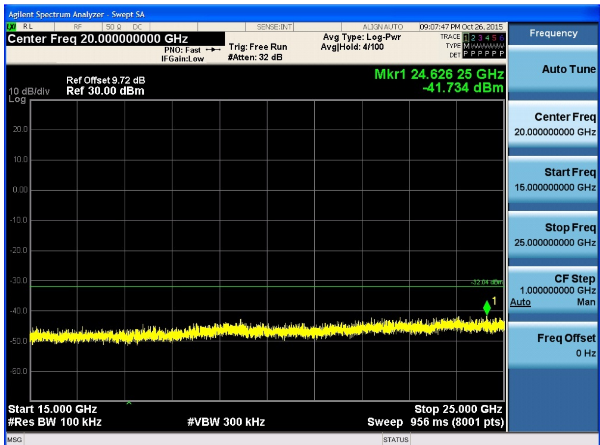
(Plot 4.6.3 A6: Channel 1: 2412MHz @ 802.11n HT20)
