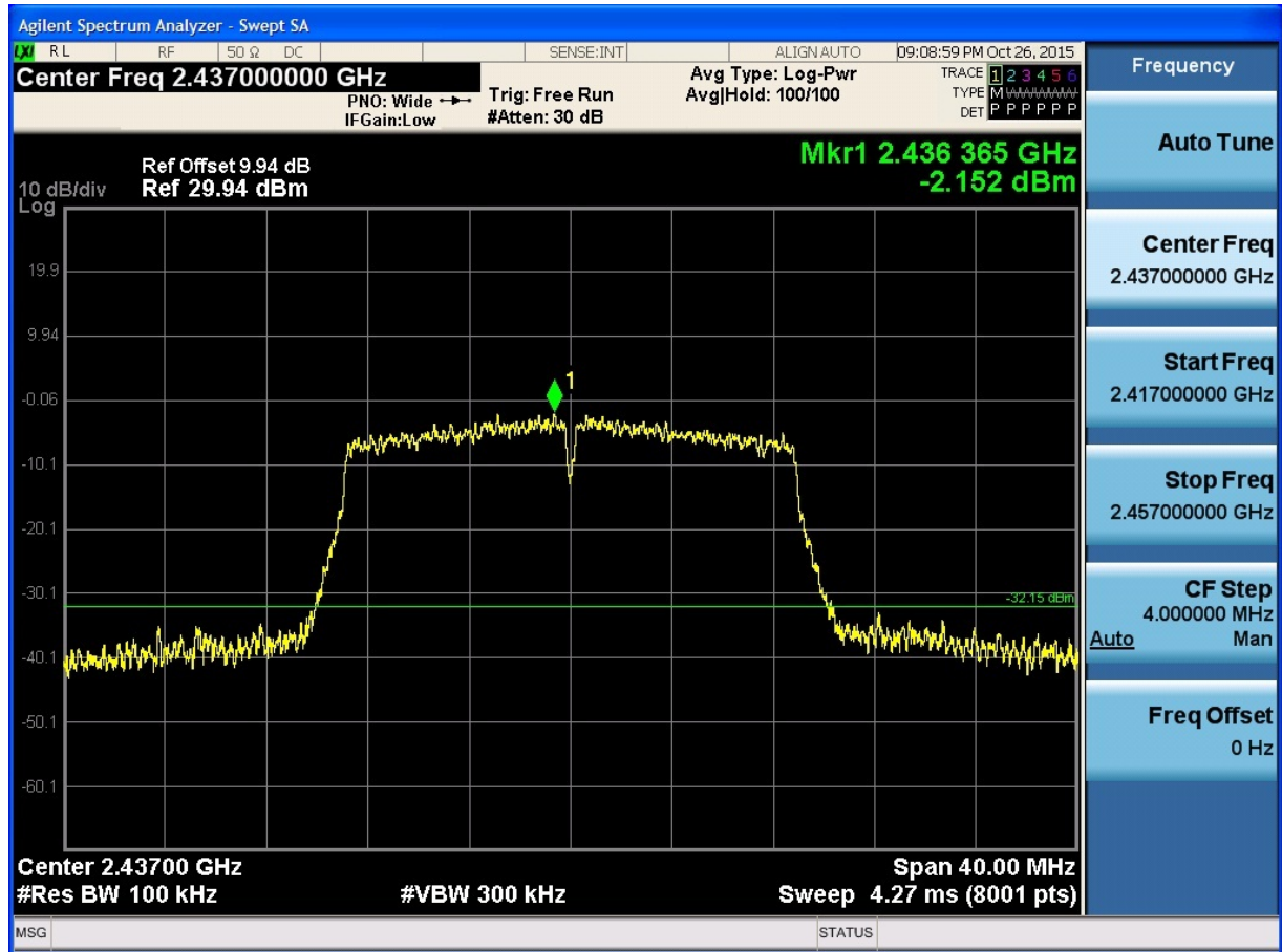
(Plot 4.6.3 B1: Channel 6: 2437MHz @ 802.11n HT20)
