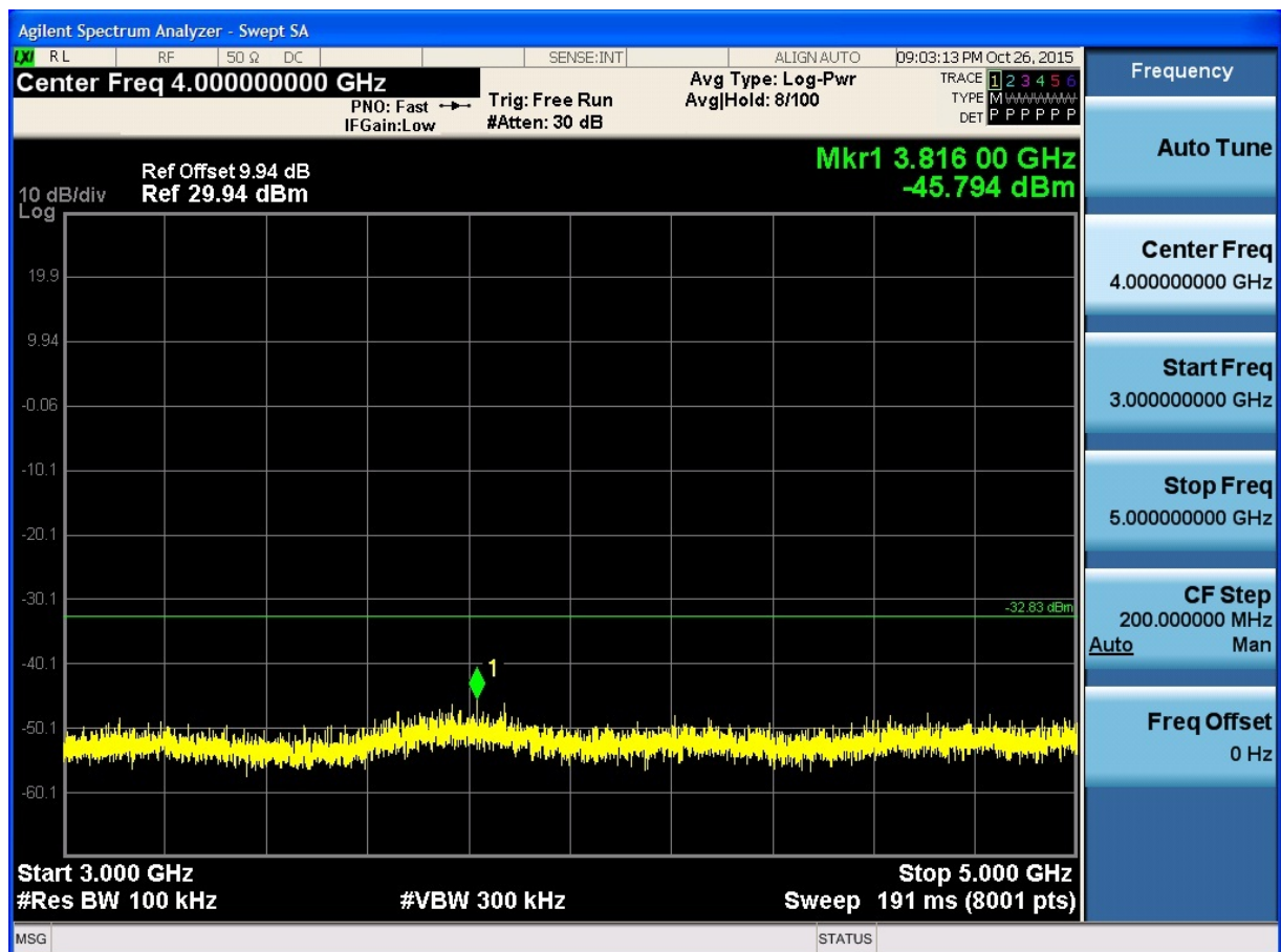
(Plot 4.6.2 B3: Channel 6: 2437MHz @ 802.11g)
