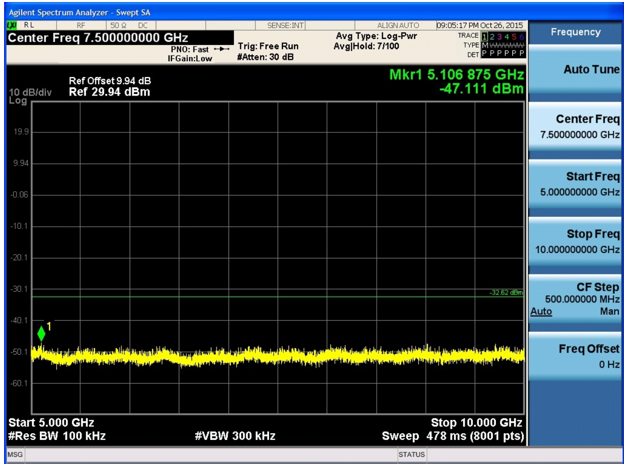
(Plot 4.6.2 C4: Channel 11: 2462MHz @ 802.11g)
