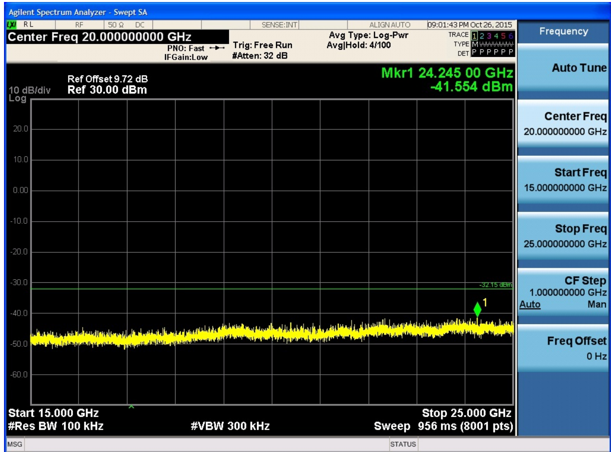
(Plot 4.6.2 A6: Channel 1: 2412MHz @ 802.11g)
