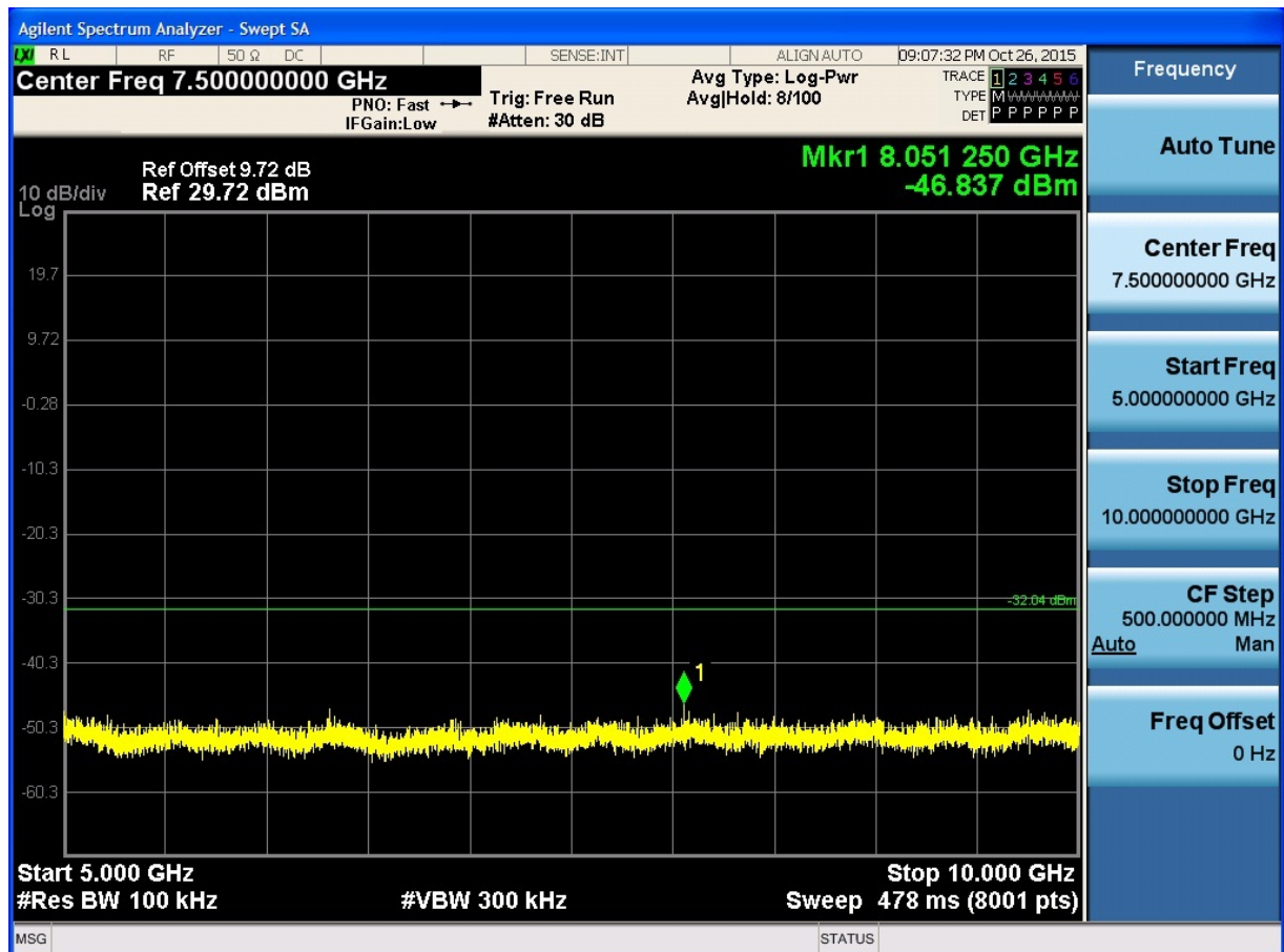
(Plot 4.6.3 A4: Channel 1: 2412MHz @ 802.11n HT20)
