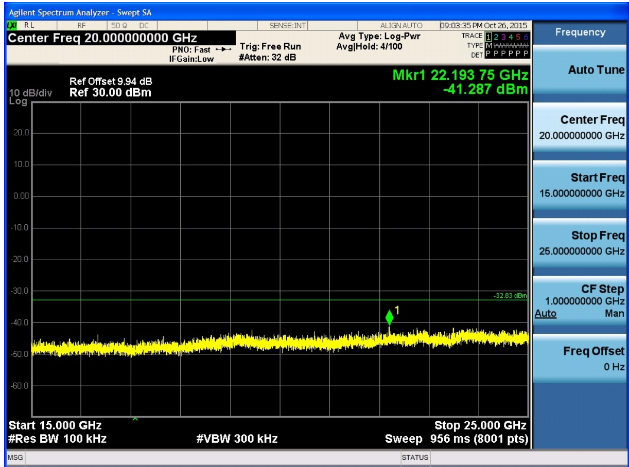
(Plot 4.6.2 B6: Channel 6: 2437MHz @ 802.11g)
