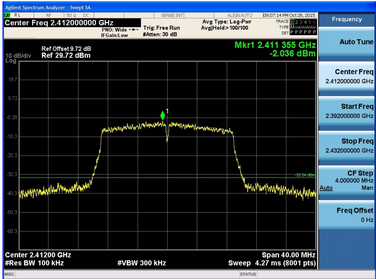
(Plot 4.6.3 A1: Channel 1: 2412MHz @ 802.11n HT20)
