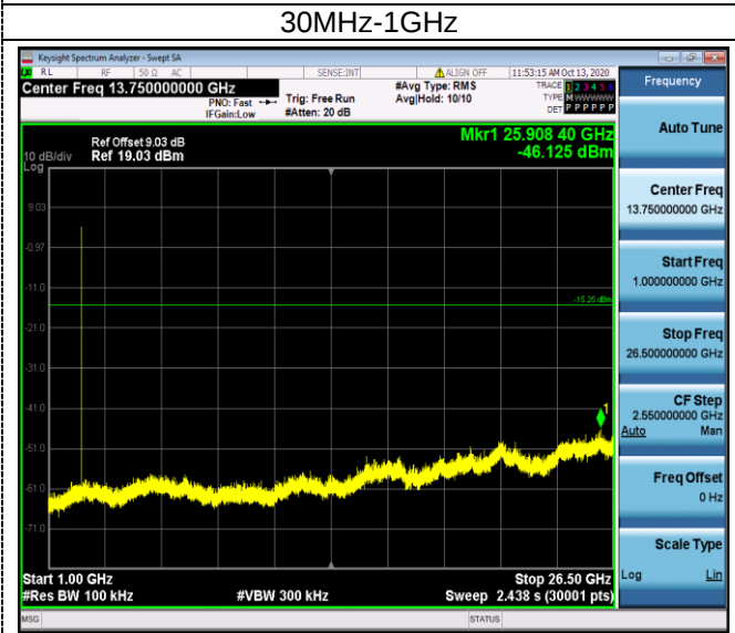
1GHz-26.5GHz
