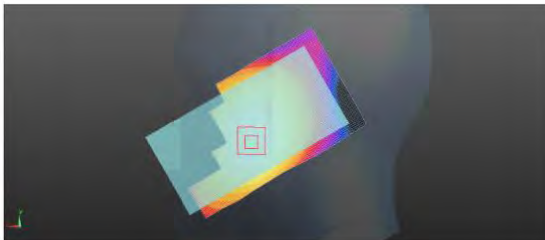
Left Head (PCS1900 Middle Channel)
