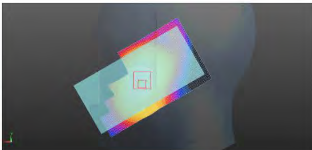
Left Head (GSM850 Middle Channel)
