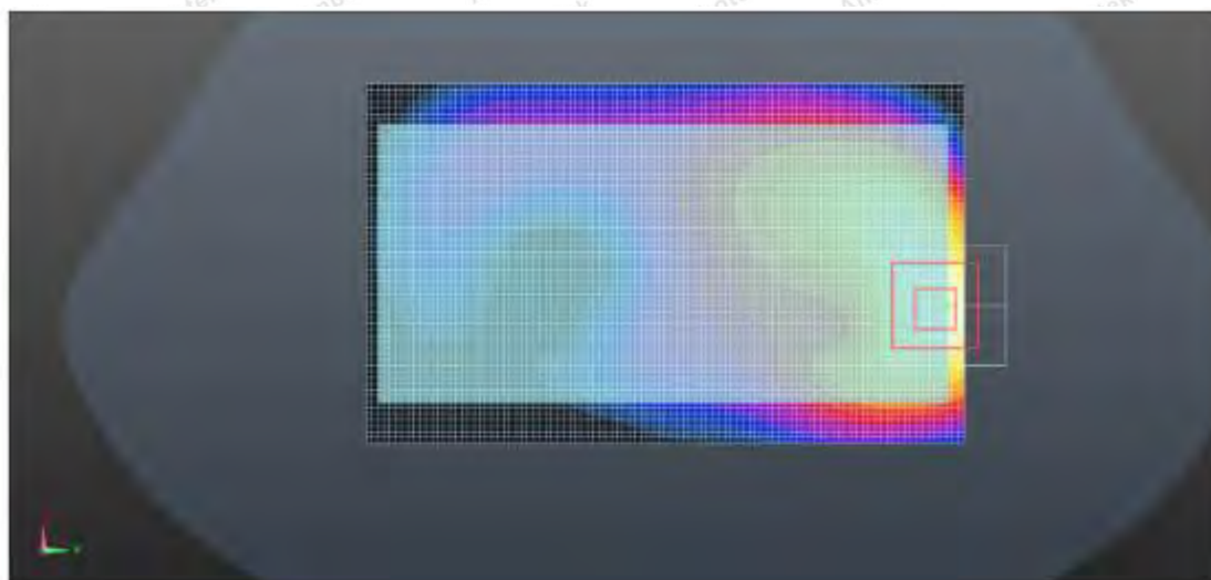
Rear Side (PCS1900 GPRS 4TS Middle Channel)
