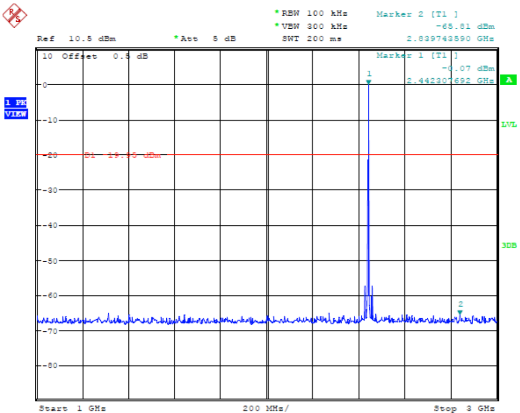
(Plot 4.6.1 B4: Channel 19: 2440MHz @ GFSK)
