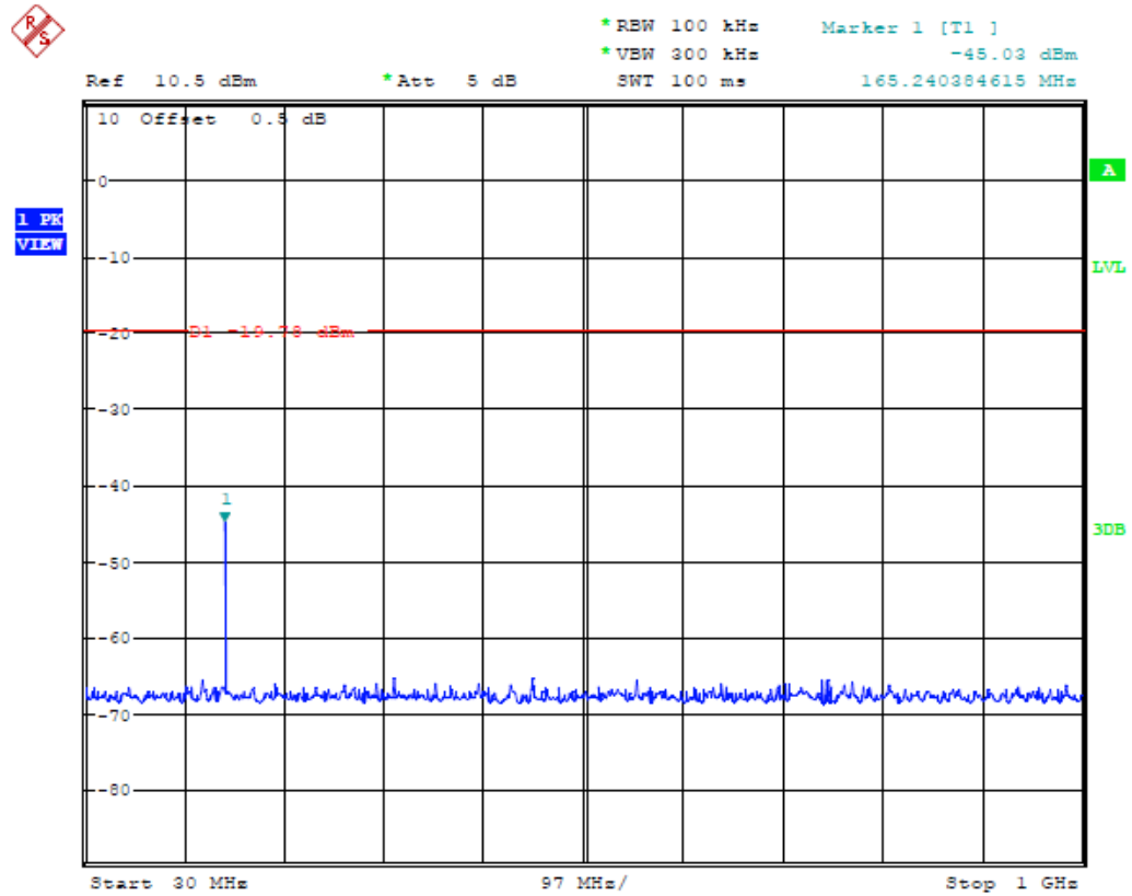
(Plot 4.6.1 C3: Channel 39: 2480MHz @ GFSK)
