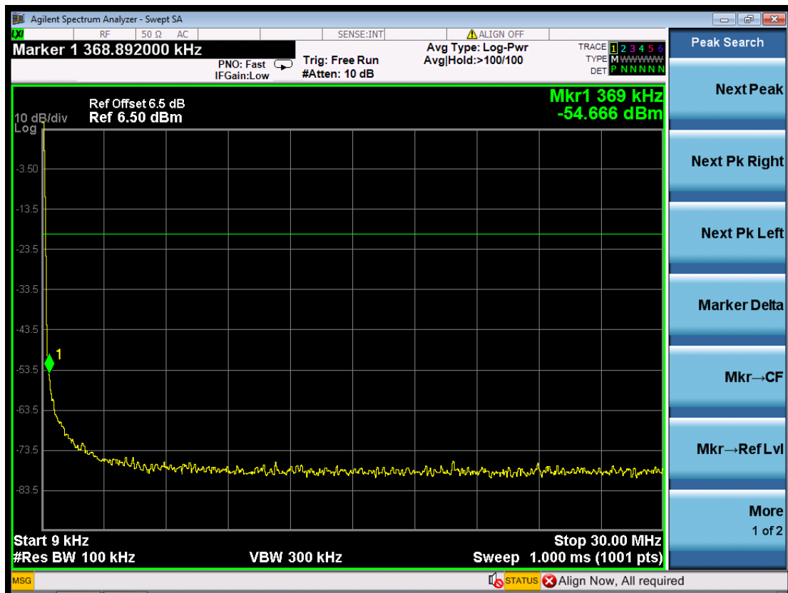
(Plot 4.6.1 A2: Channel 00: 2402MHz @ GFSK)
