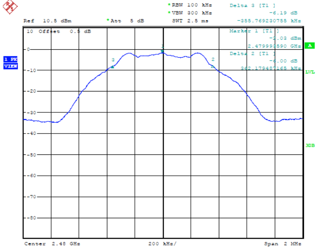
(Plot 4.7.1 C: Channel 39: 2480MHz @ GFSK)
