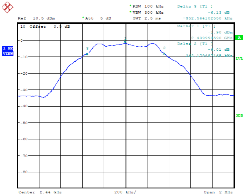
(Plot 4.7.1 B: Channel 19: 2440MHz @ GFSK)
