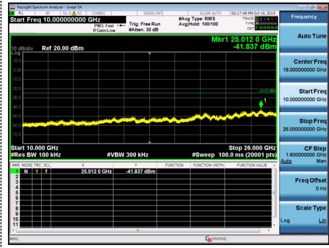
10GHz-26GHz
