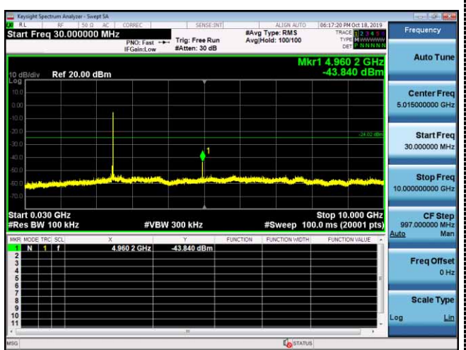
30MHz-10GHz
