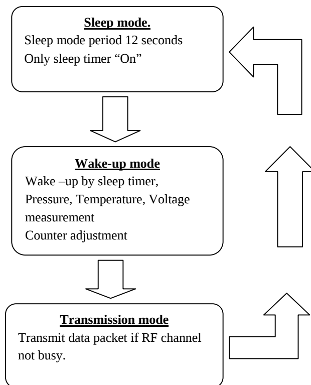
Pic.1 CBTPSEN01 operation flow chart.
