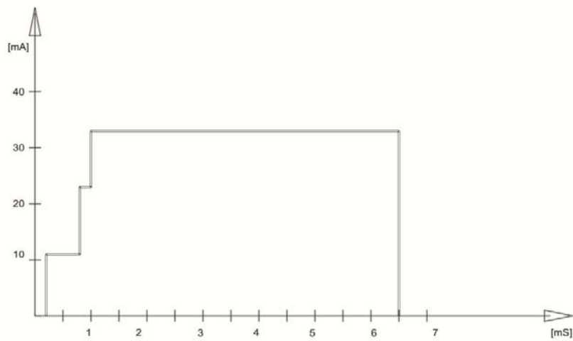
Pic.2 CBTPSEN01 active period.
