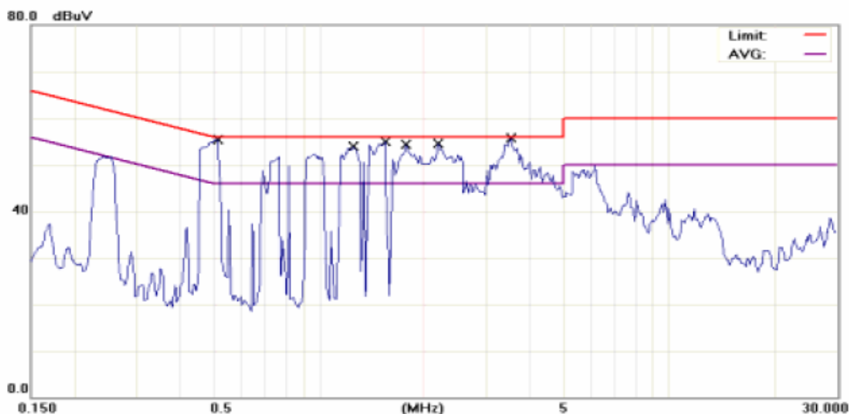
Conducted Emission Measurement
