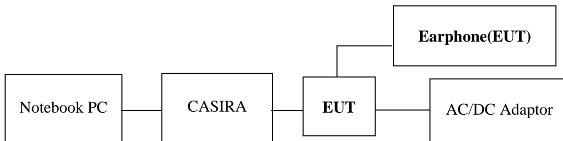
Fig. 2-1 Configuration of Tested System
