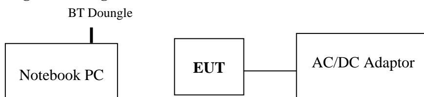
Fig. 2-2 Configuration of AC Power Line Conducted Emission
