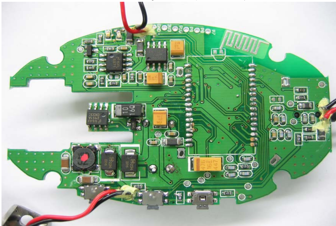
Internal View of EUT – 2 (KBT120N-5)
