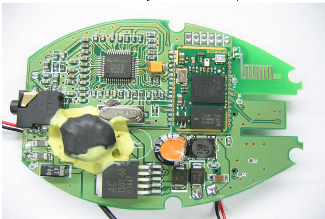
Internal View of EUT – 2 (KBT120N-6)
