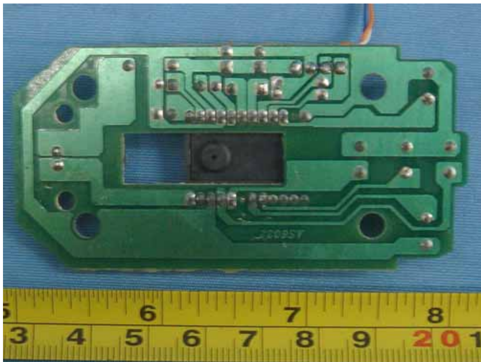
PCB - Solder View
