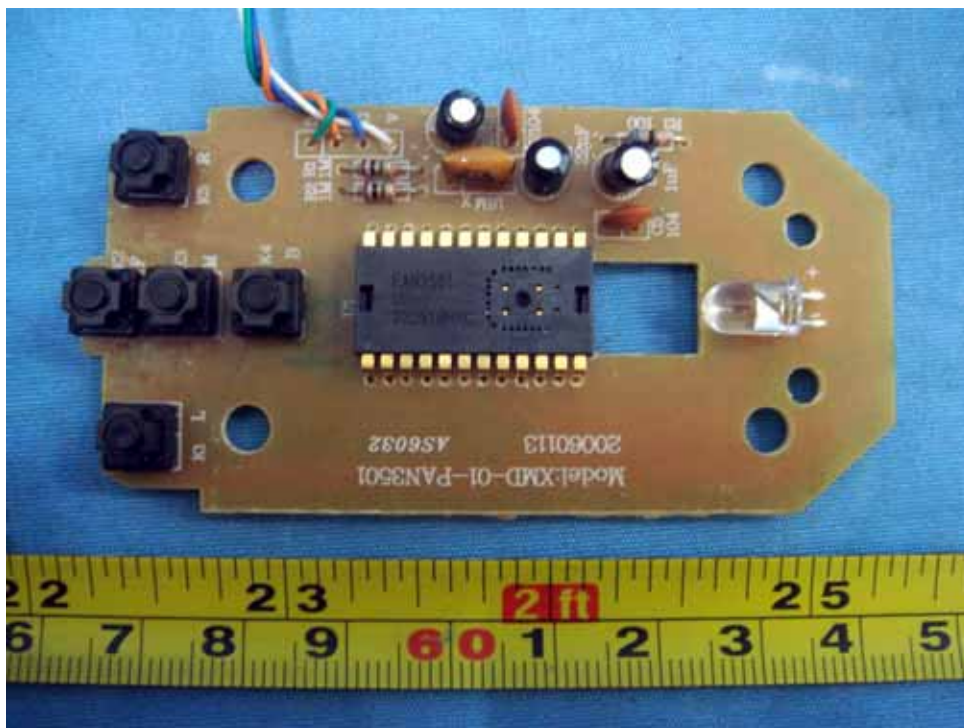
PCB - Component View
