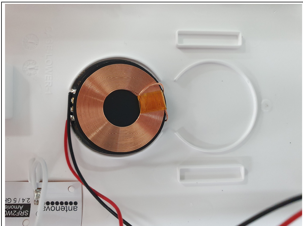
<Coil Antenna>
