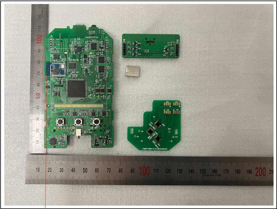
BT/BLE Antenna
