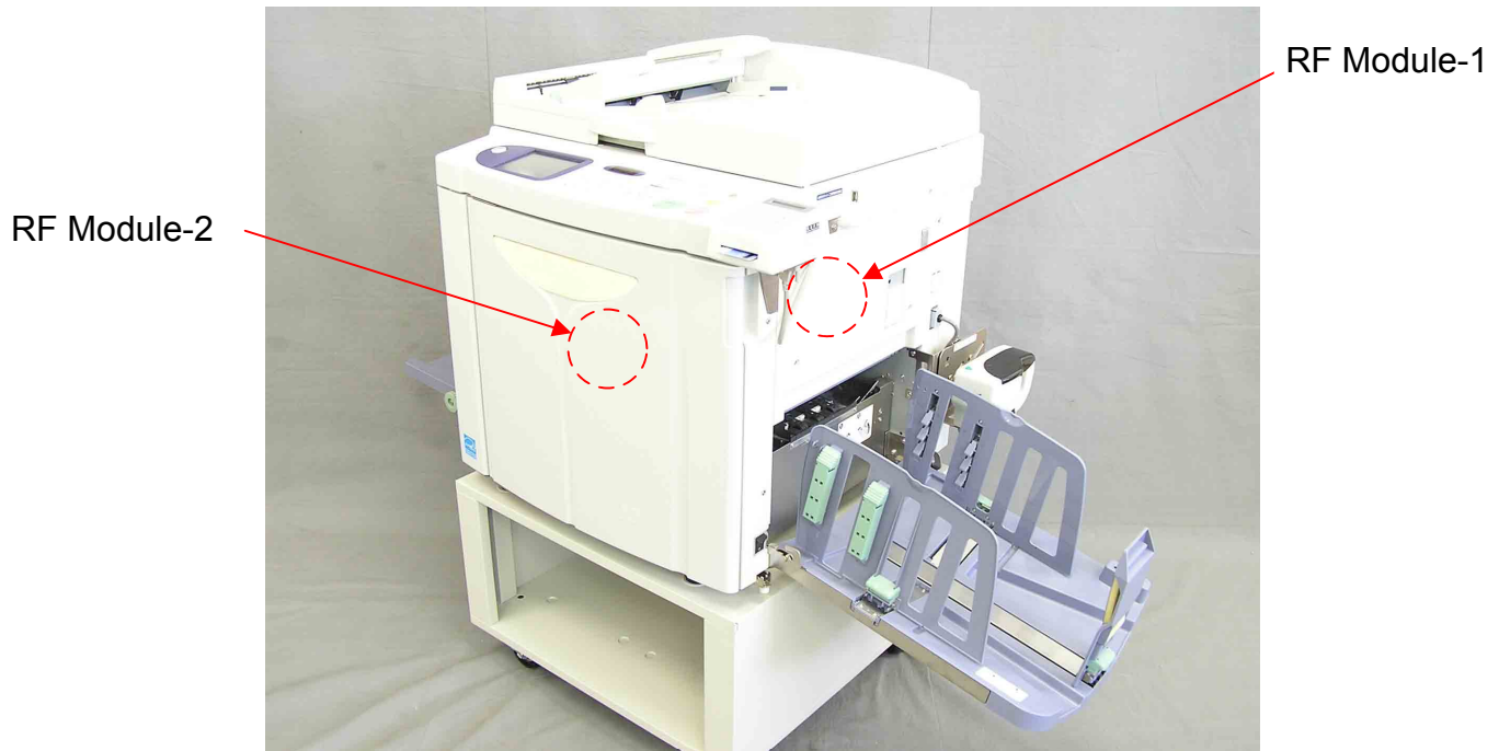
Host Device
