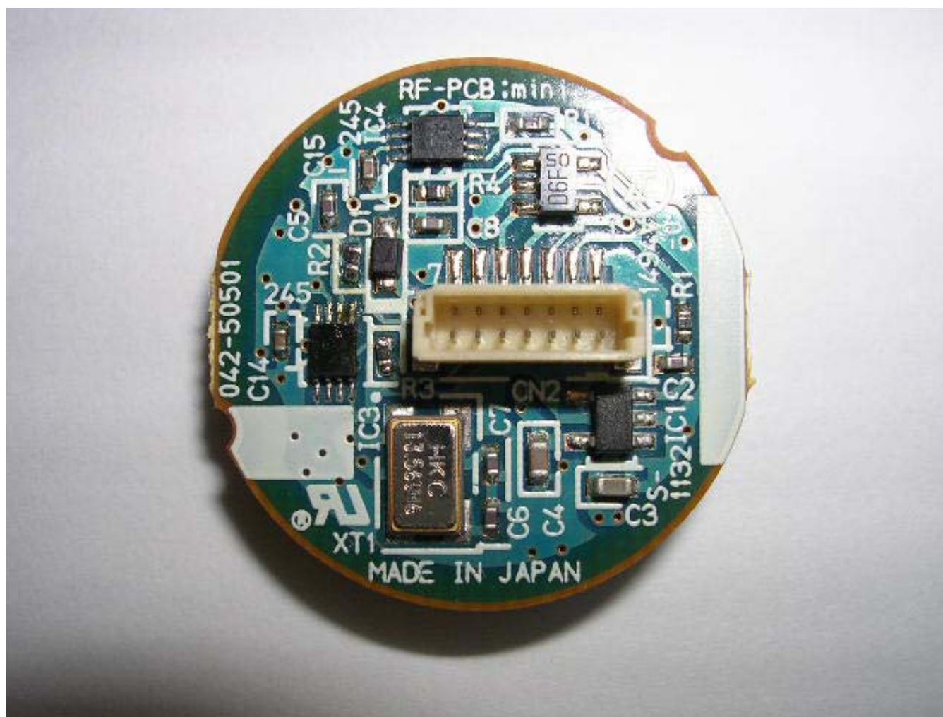
042-50501 (RF-MODULE-V4) Component side
