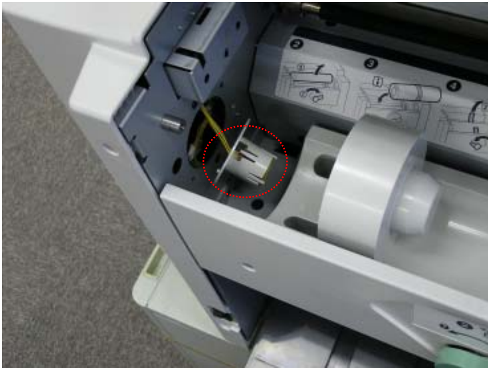
Photo3: Location of RF Module-2 (RF Module-2 is fixed with a columnar fixed material.)
