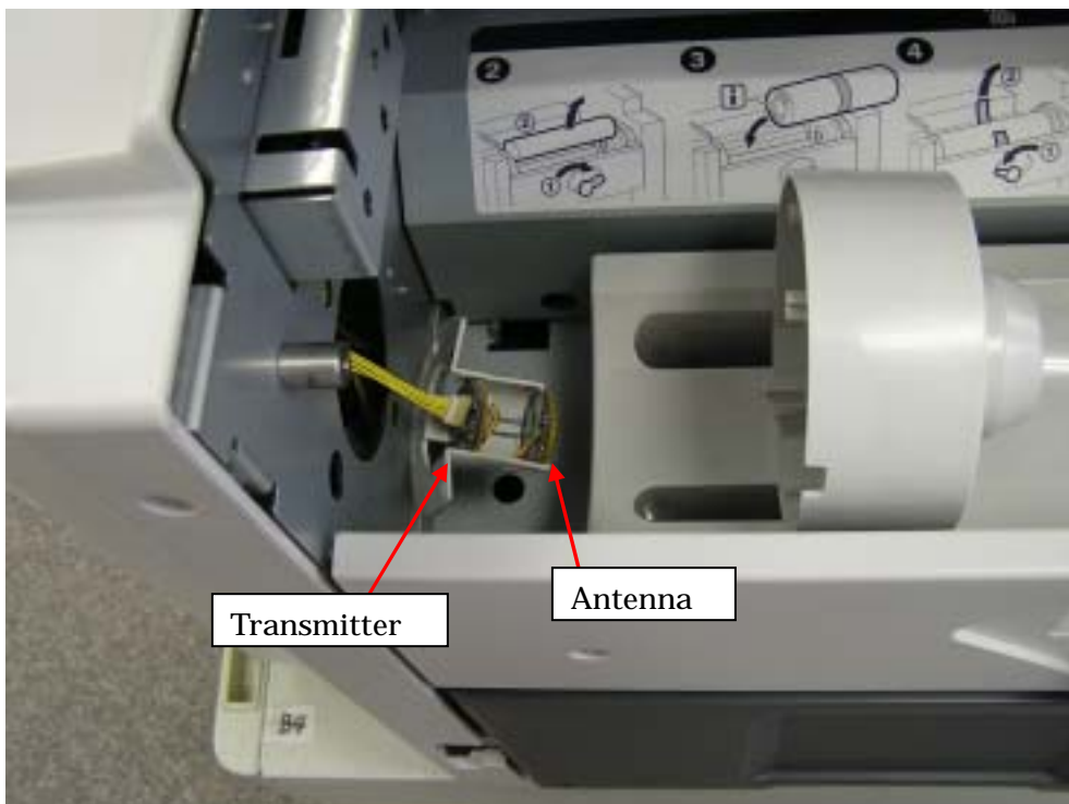
Photo4: Cut the fixed material to show how RF Module-2 is installed into a host device
