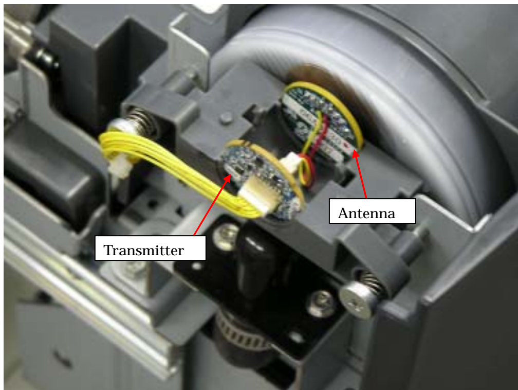
Photo4: Open the fixed material to show how RF Module-1 is installed into a host device
