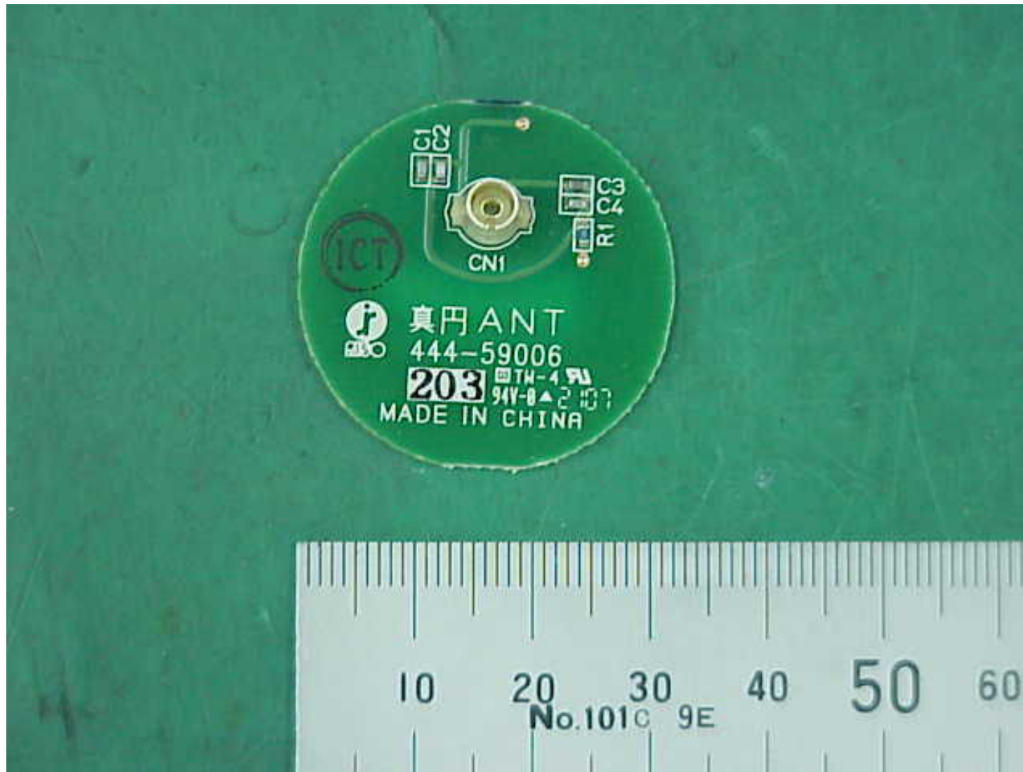
O-Shape Antenna ( 444-59006 ) Parts Side
