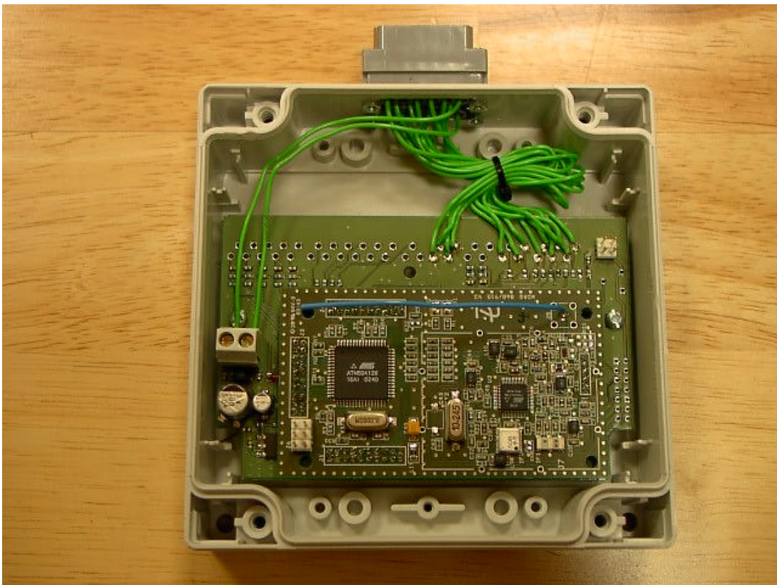
Control unit
