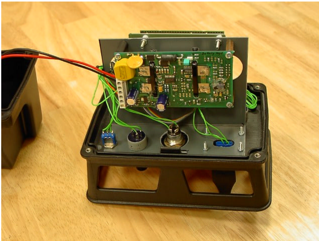
Handheld unit
