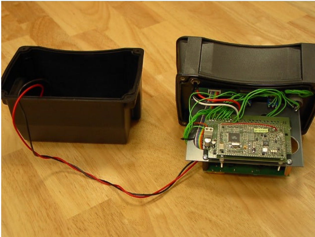
Handheld unit
