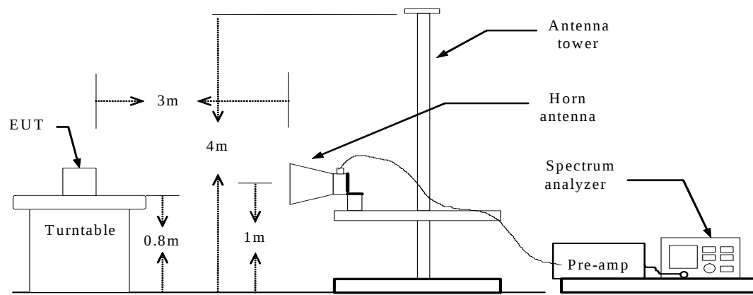
Above 1 GHz
