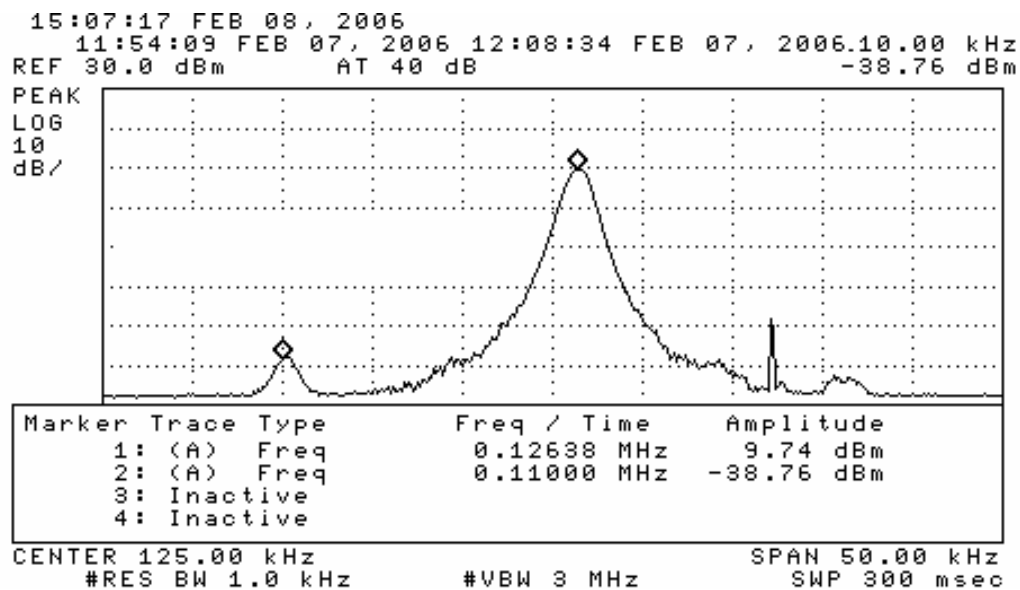
Figure 6.3. Measured bandwidth of the DUT.
