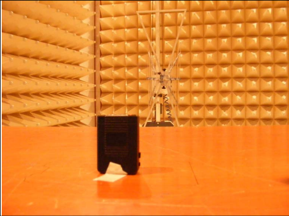
A. Photo of Field Strength & Spurious Emission Test
