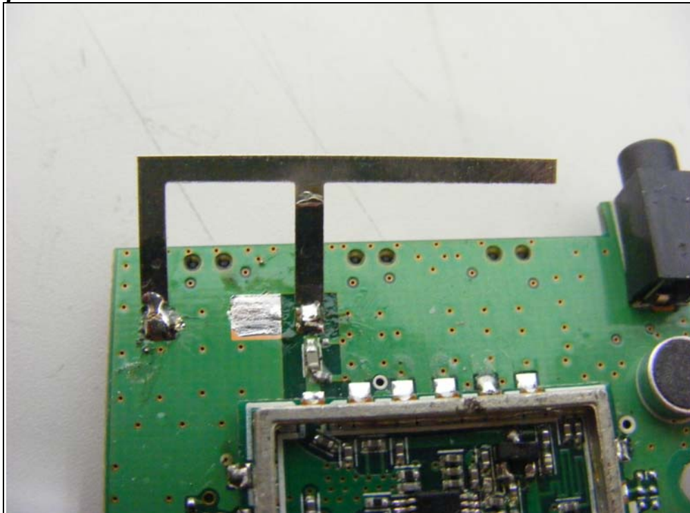
Antenna of EUT
