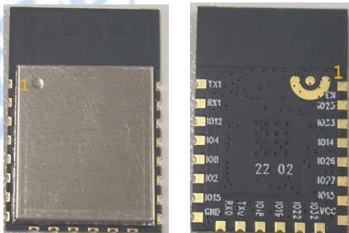
PCBA physical photo
