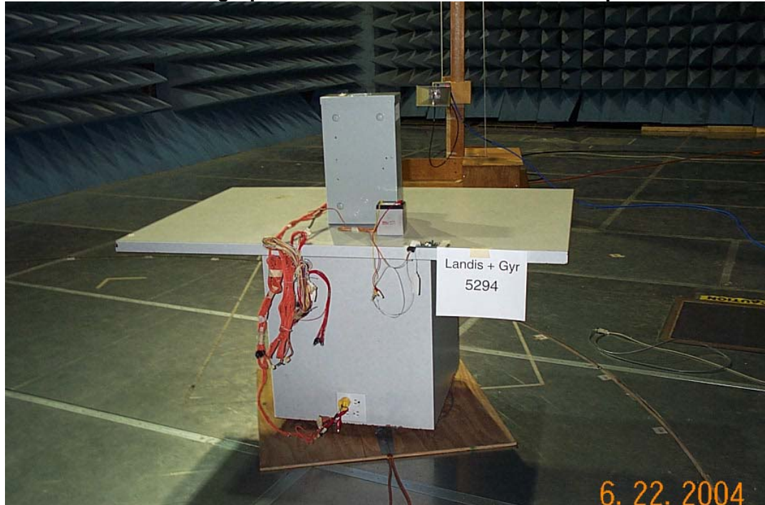
Photograph of Radiated Emissions Test Setup
