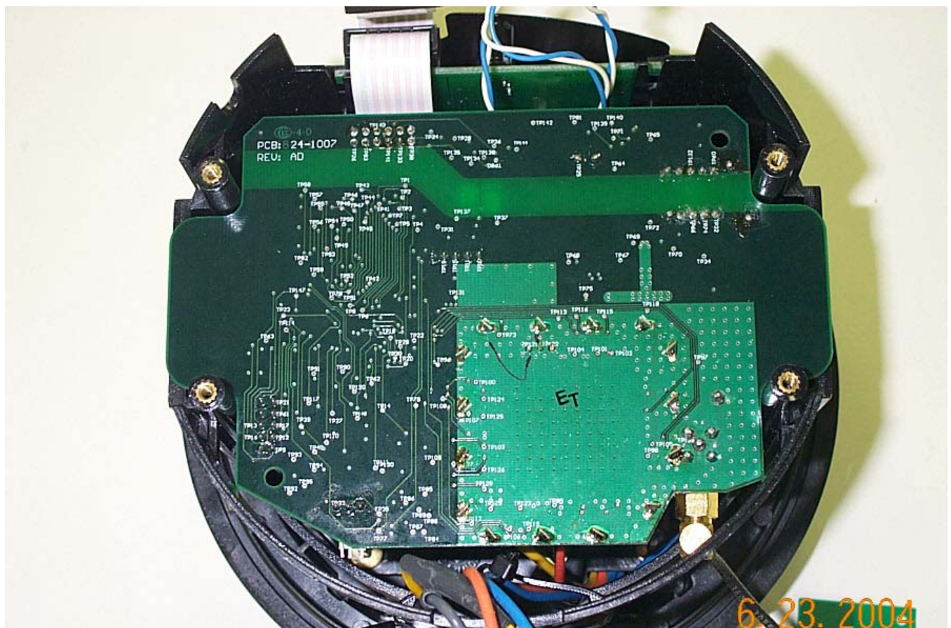
Transceiver Installed in meter
