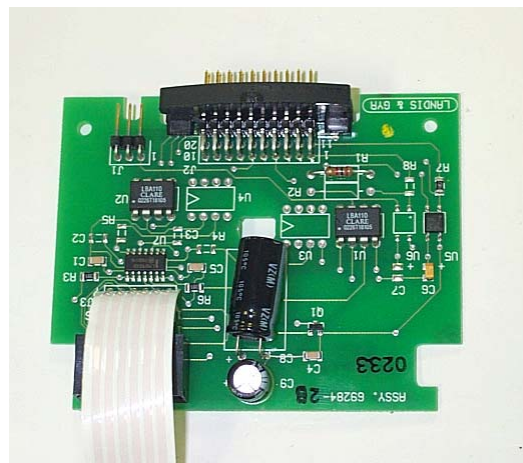
Component side
