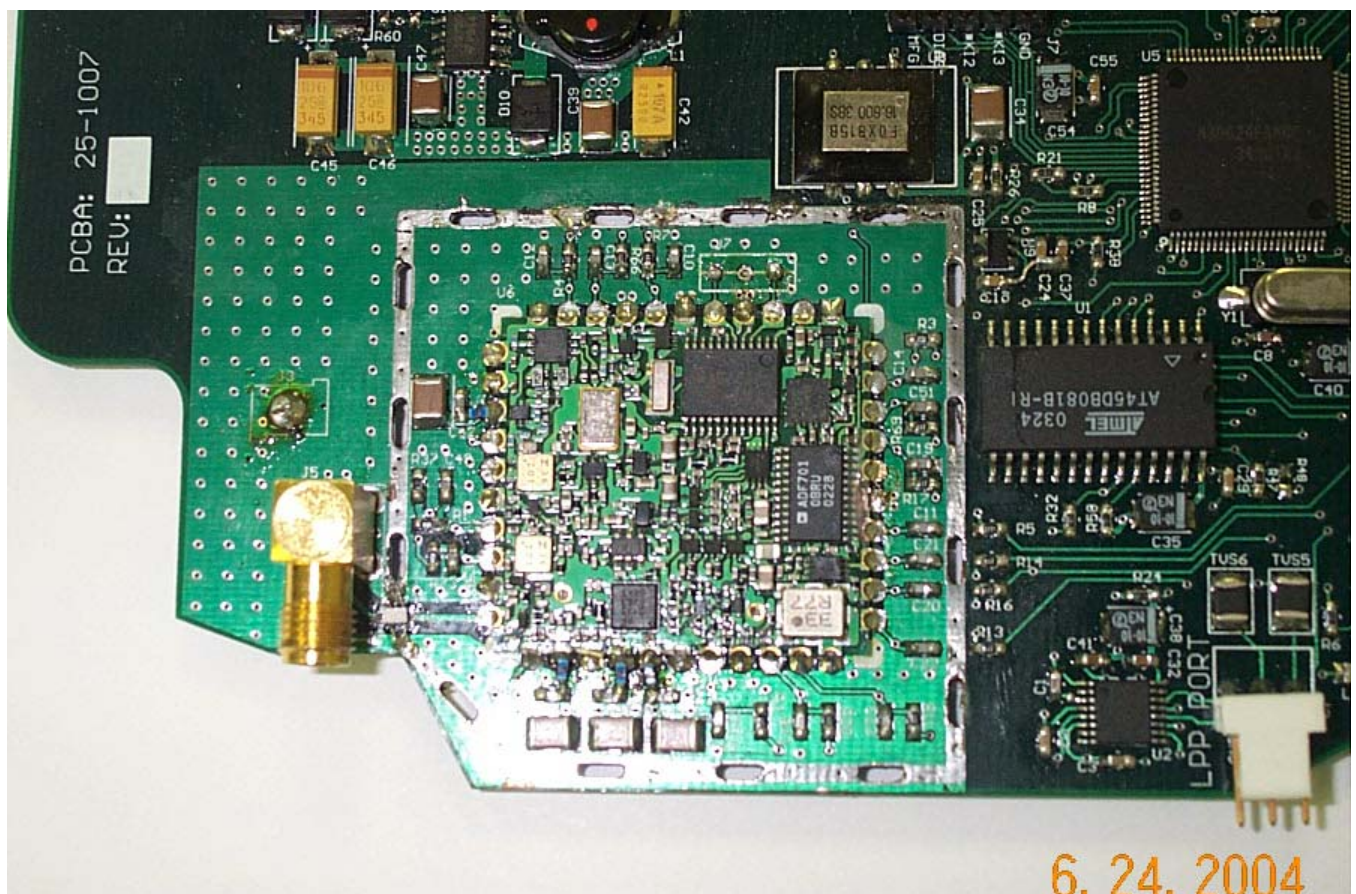
Transceiver PCB with RF shields removed. This shows the circuitry under the metal shield.
