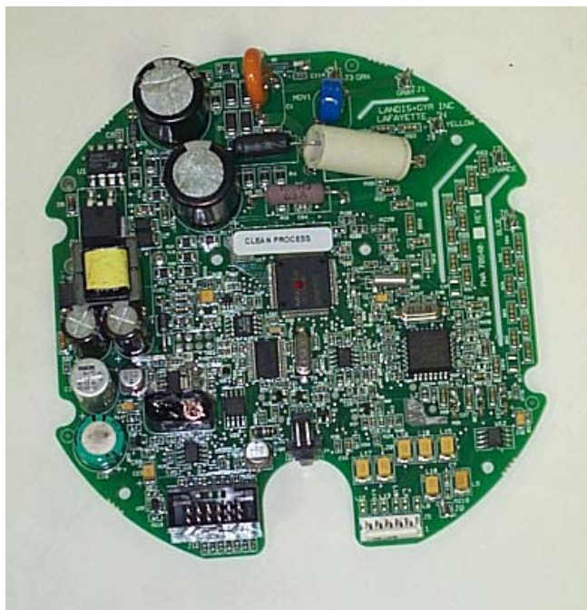
Electricity meter PCB; component side
