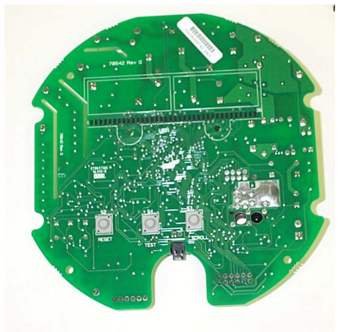
Foil side
