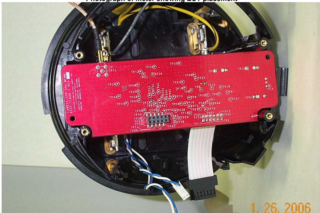
Photograph of meter showing EUT placement
