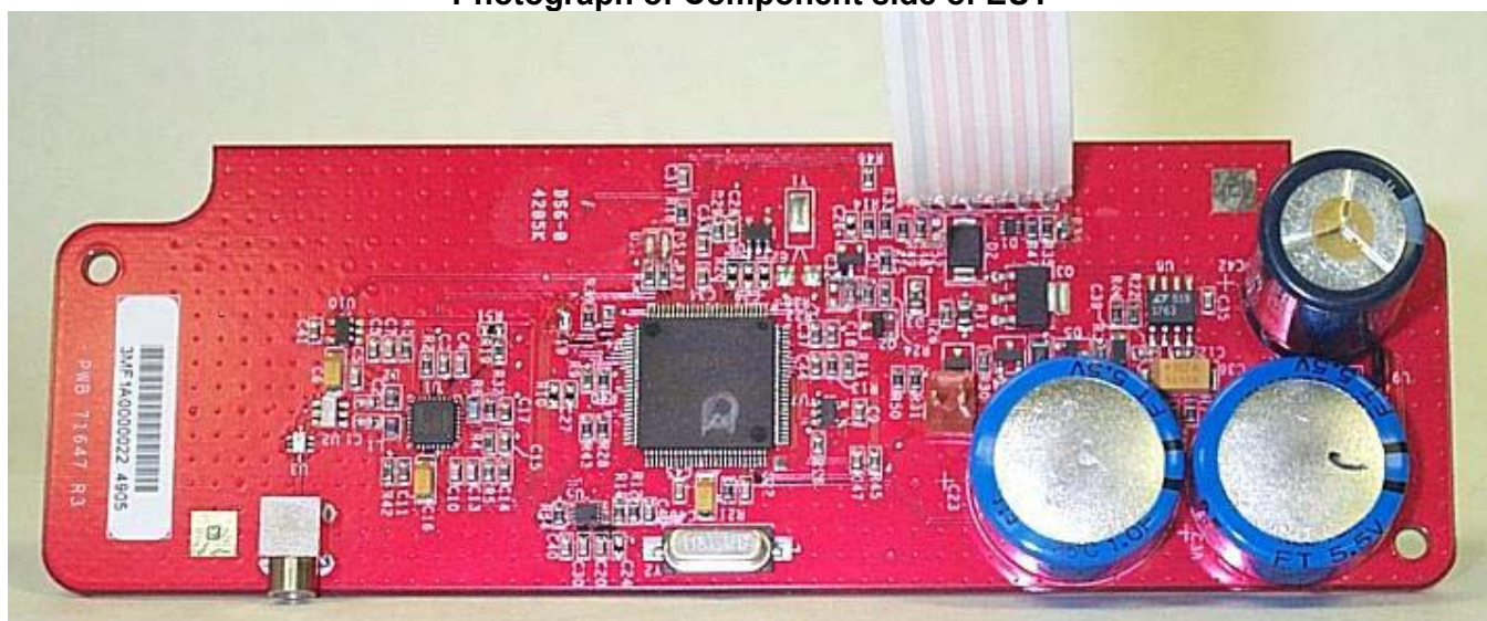
Photograph of Component side of EUT
