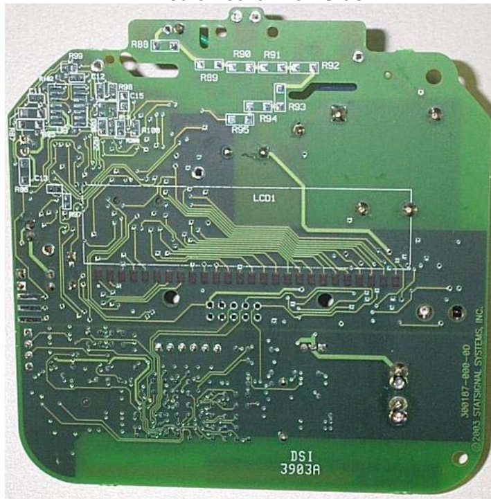
Circuit Board: Foil Side
