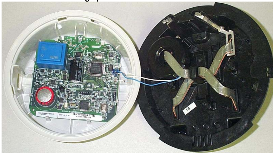
Photograph of EUT Front Cover Removed
