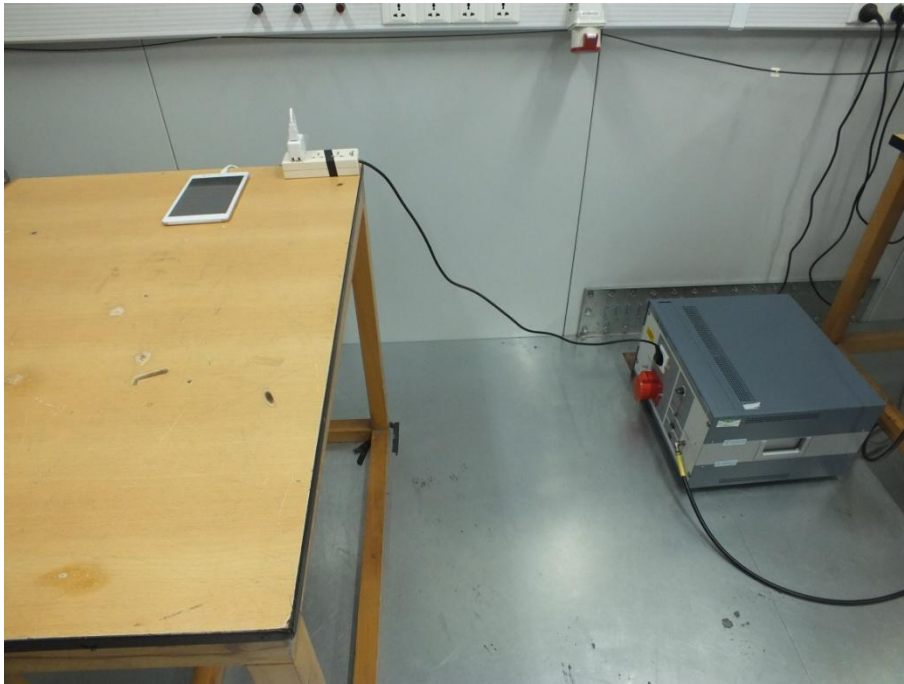
AC Conducted Emission Test Setup
