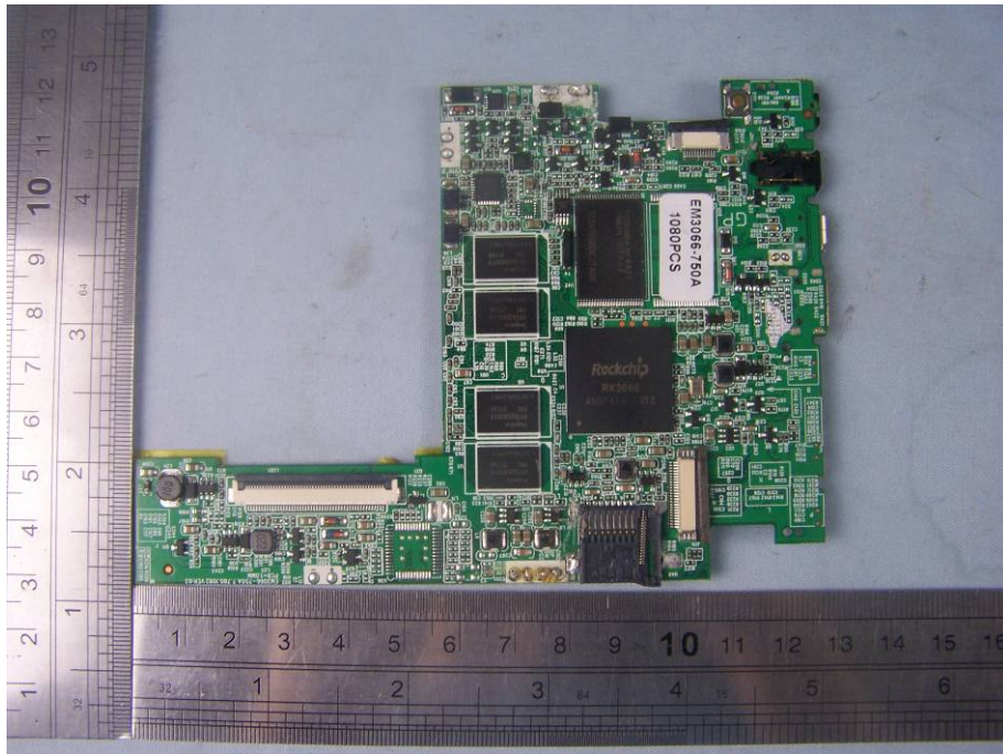
Main board2# -Top View
