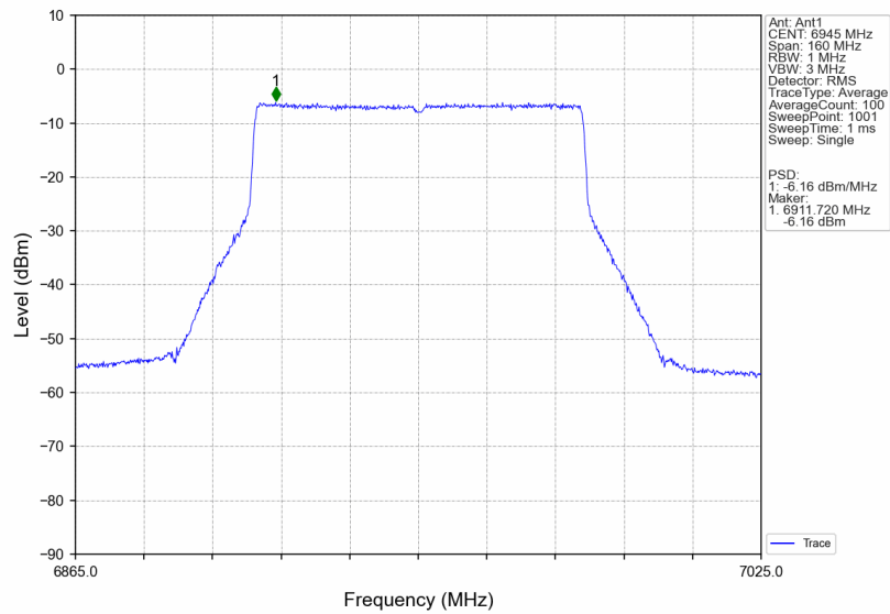
802.11ax(VHT80)_LCH_6945MHz_Ant1_NTNV
