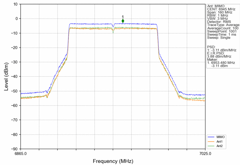
802.11ax(VHT80)_LCH_6945MHz_MIMO_NTNV
