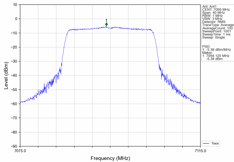
802.11ax(VHT20)_HCH_7095MHz_Ant1_NTNV
