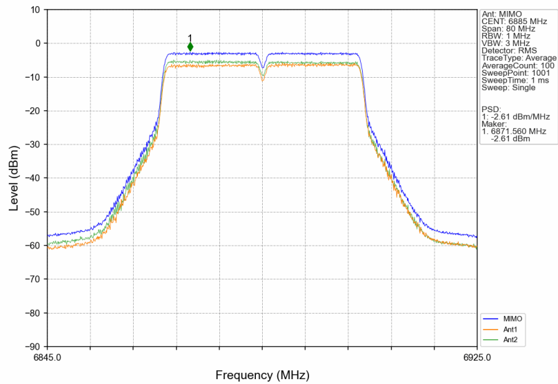
802.11ax(VHT40)_HCH_6885MHz_MIMO_NTNV
