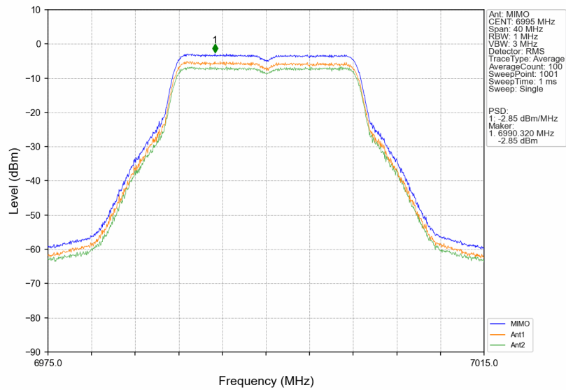
802.11ax(VHT20)_MCH_6995MHz_MIMO_NTNV
