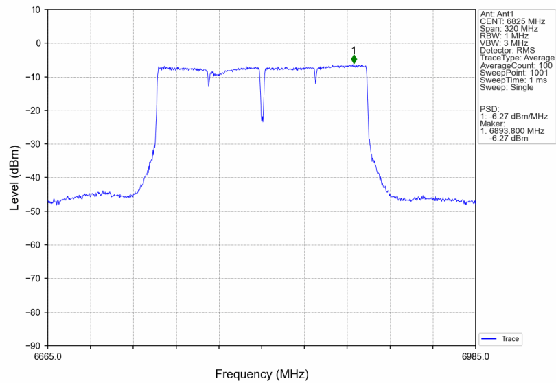
802.11ax(VHT160)_HCH_6825MHz_Ant1_NTNV
