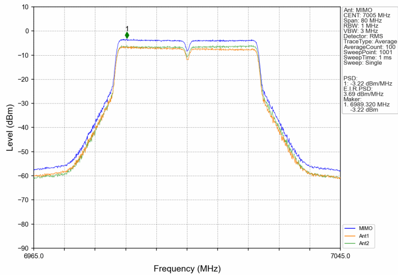
802.11ax(VHT40)_MCH_7005MHz_MIMO_NTNV
