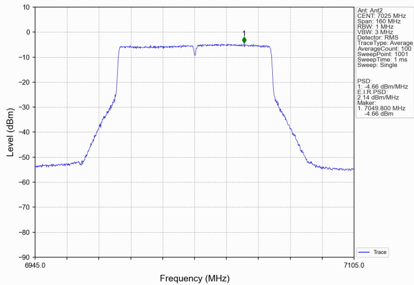
802.11ax(VHT80)_HCH_7025MHz_Ant2_NTNV
