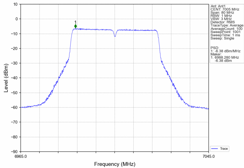
802.11ax(VHT40)_MCH_7005MHz_Ant1_NTNV
