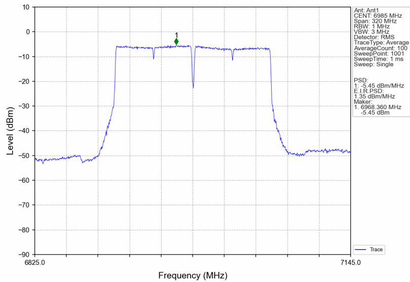
802.11ax(VHT160)_MCH_6985MHz_Ant1_NTNV
