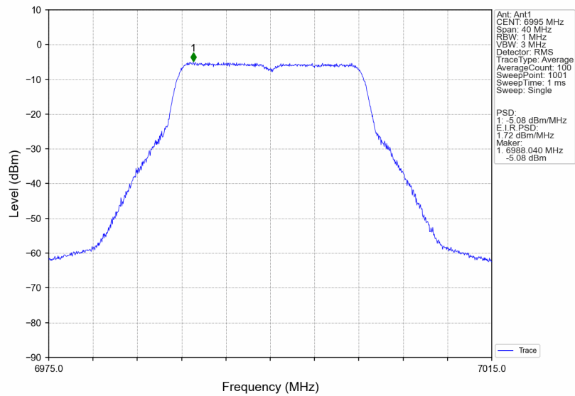
802.11ax(VHT20)_MCH_6995MHz_Ant1_NTNV
