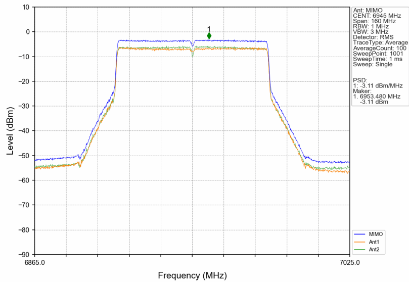
802.11ax(VHT80)_LCH_6945MHz_MIMO_NTNV
