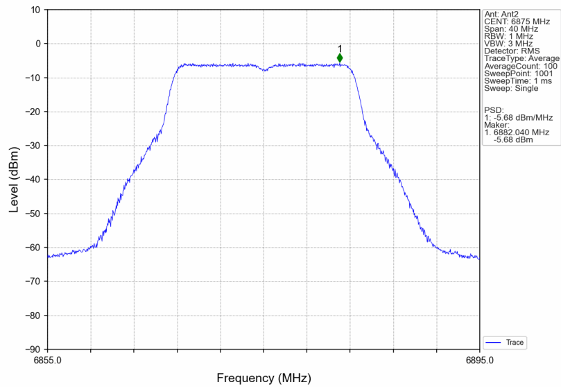
802.11ax(VHT20)_HCH_6875MHz_Ant2_NTNV
