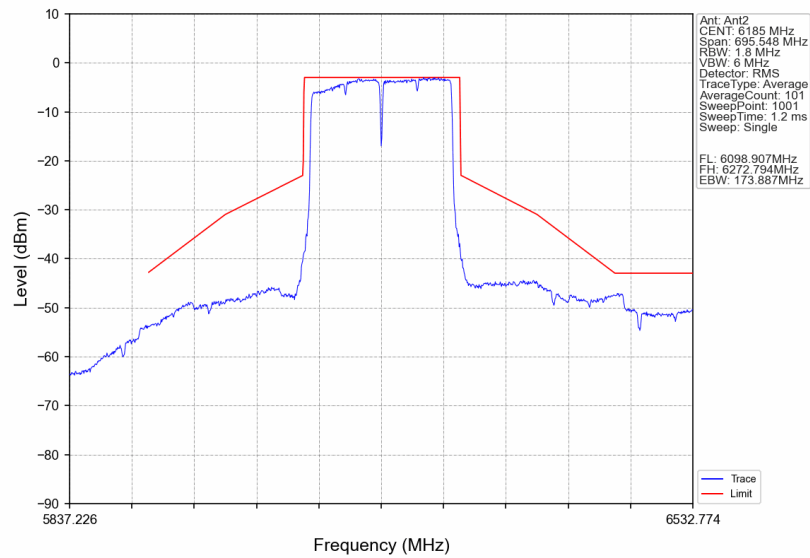
802.11ax(VHT160)_MCH_6185MHz_Ant2_NTNV
