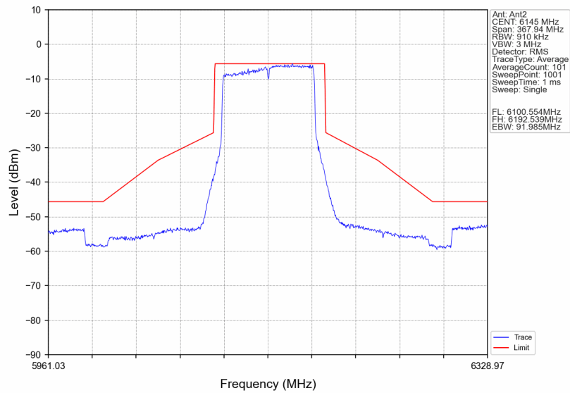
802.11ax(VHT80)_MCH_6145MHz_Ant2_NTNV
