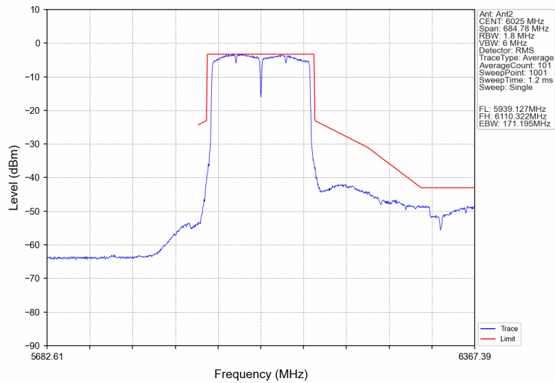
802.11ax(VHT160)_LCH_6025MHz_Ant2_NTNV
