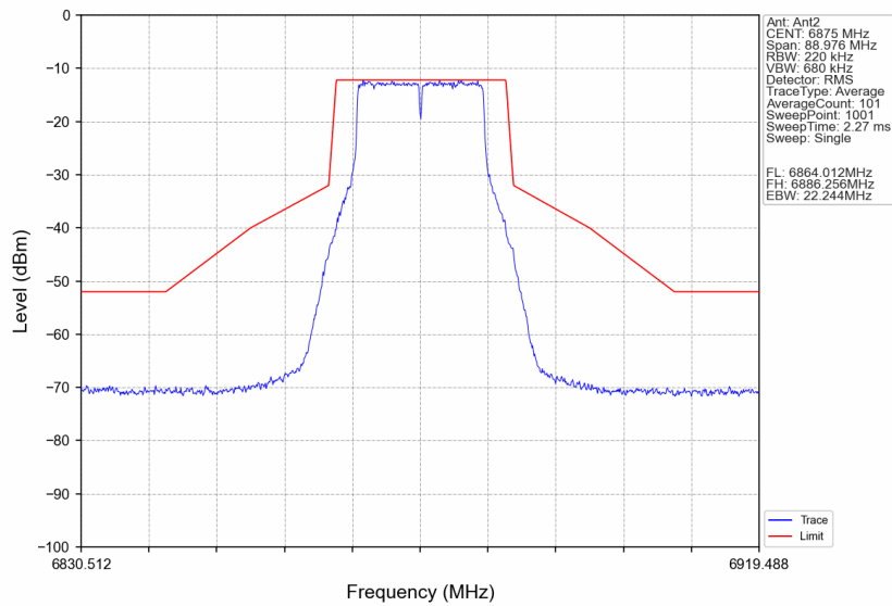
802.11ax(VHT20)_HCH_6875MHz_Ant2_NTNV
