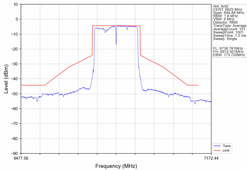
802.11ax(VHT160)_HCH_6825MHz_Ant2_NTNV
