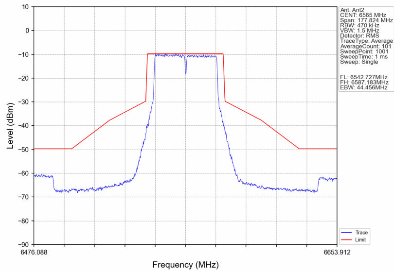
802.11ax(VHT40)_LCH_6565MHz_Ant2_NTNV
