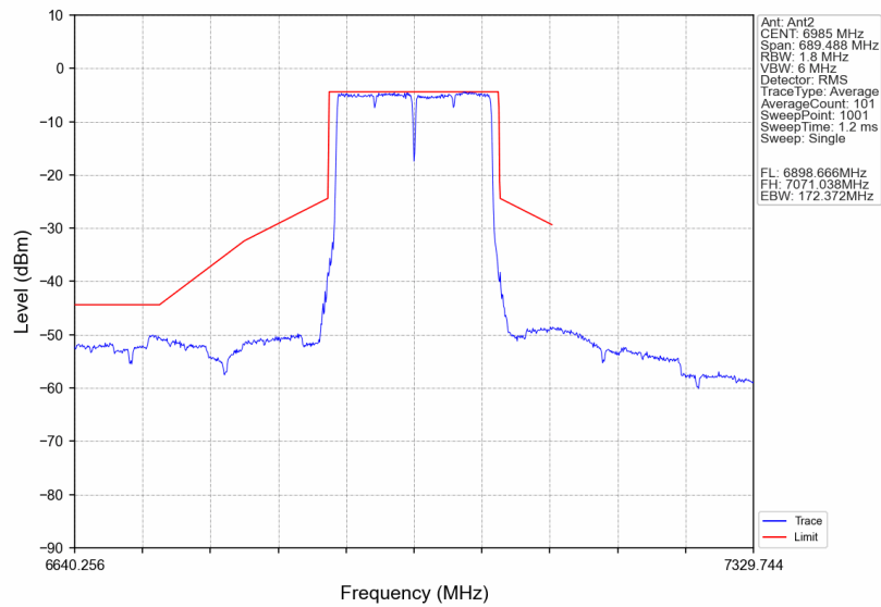
802.11ax(VHT160)_MCH_6985MHz_Ant2_NTNV
