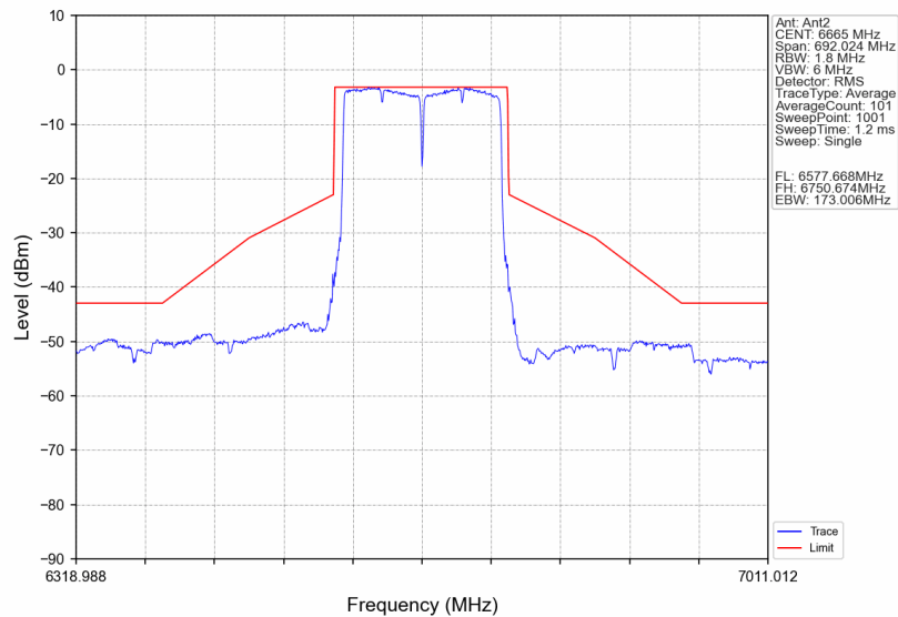
802.11ax(VHT160)_MCH_6665MHz_Ant2_NTNV
