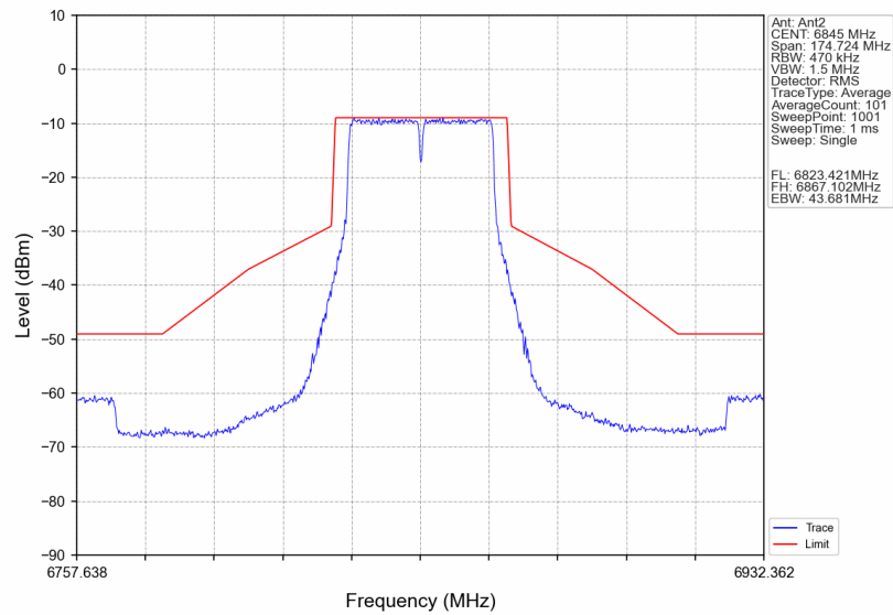
802.11ax(VHT40)_HCH_6845MHz_Ant2_NTNV
