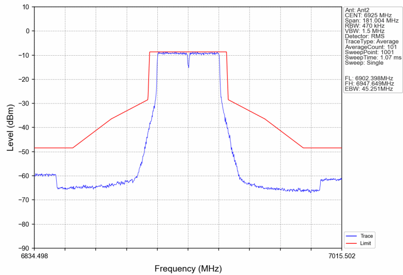
802.11ax(VHT40)_LCH_6925MHz_Ant2_NTNV
