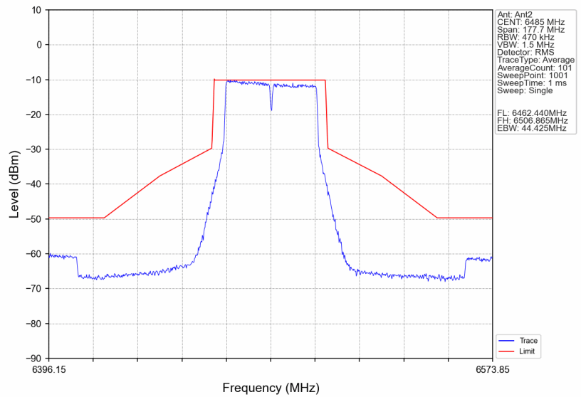
802.11ax(VHT40)_MCH_6485MHz_Ant2_NTNV
