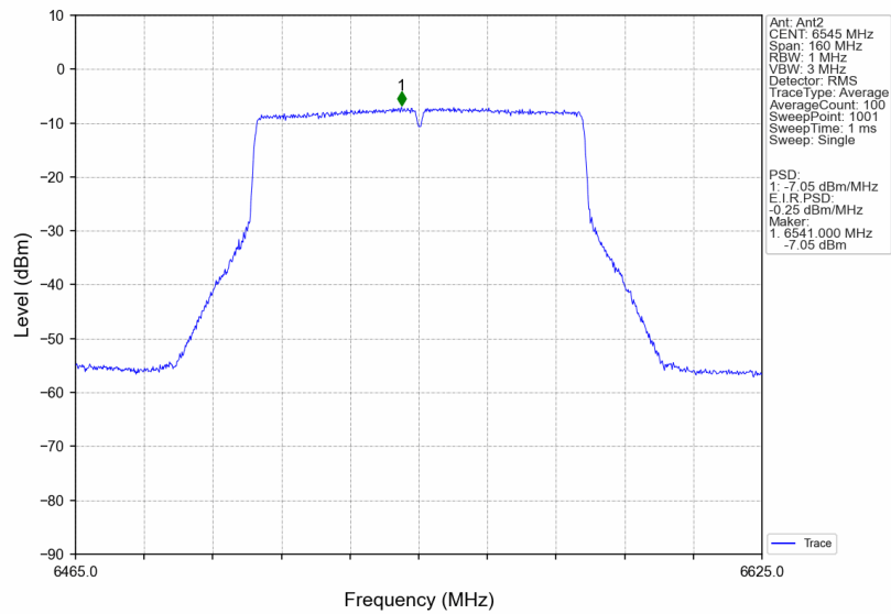
802.11ax(VHT80)_HCH_6545MHz_MIMO_NTNV
