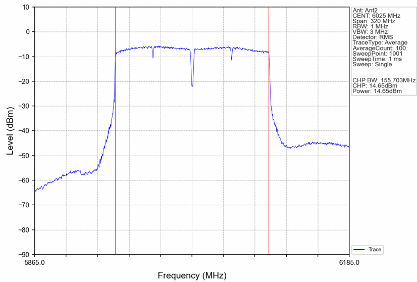
802.11ax(VHT160)_LCH_6025MHz_Ant2_NTNV
