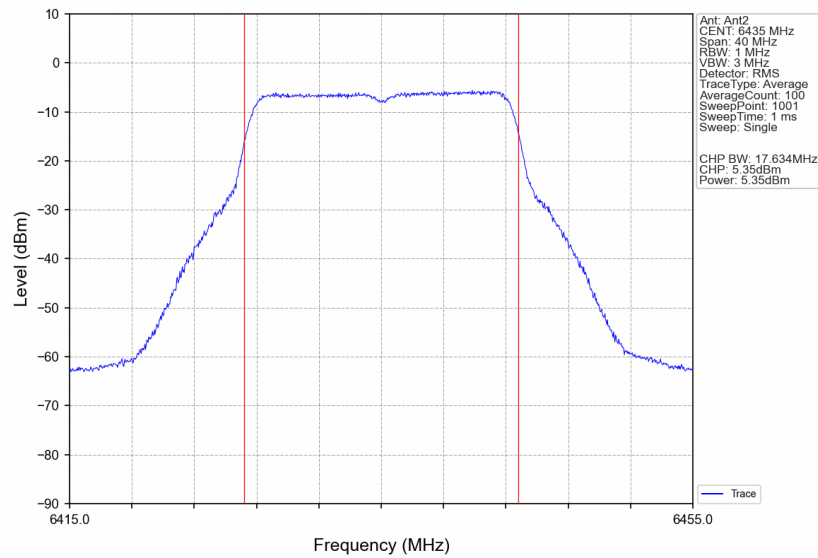
802.11ax(VHT20)_LCH_6435MHz_Ant2_NTNV
