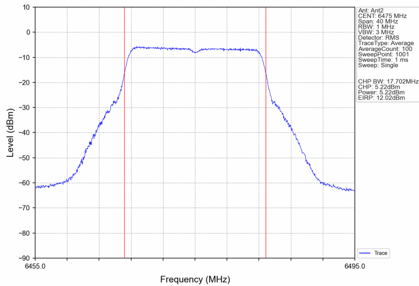
802.11ax(VHT20)_MCH_6475MHz_Ant2_NTNV
