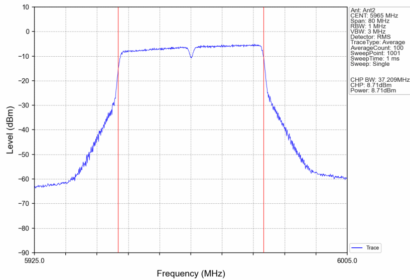
802.11ax(VHT40)_LCH_5965MHz_Ant2_NTNV
