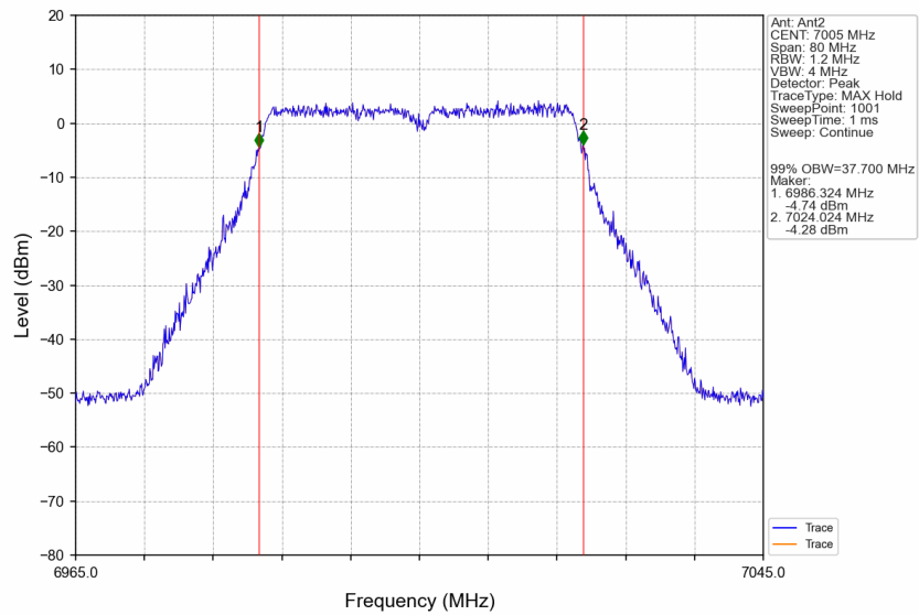
802.11ax(VHT40)_MCH_7005MHz_Ant2_NTNV
