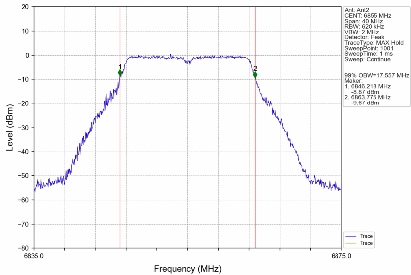
802.11ax(VHT20)_HCH_6855MHz_Ant2_NTNV
