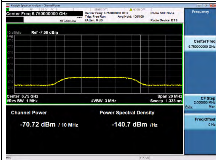
11BE320SISO-Ant 1-6905-Center-6750-Minimal
