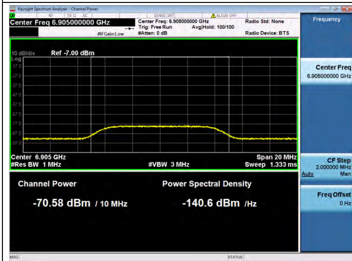
11BE320SISO-Ant 1-6905-Center-6905-Minimal
