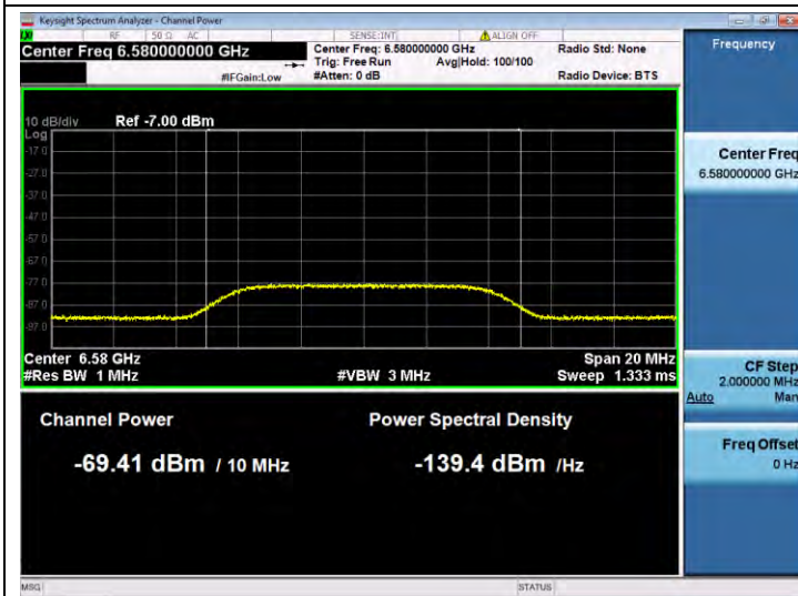
11BE320SISO-Ant 1-6425-Center-6580-Minimal
