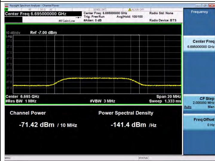
11BE20SISO-Ant 1-6695-Center-6695-Minimal
