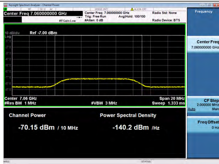
11BE320SISO-Ant 1-6905-Center-7060-Minimal
