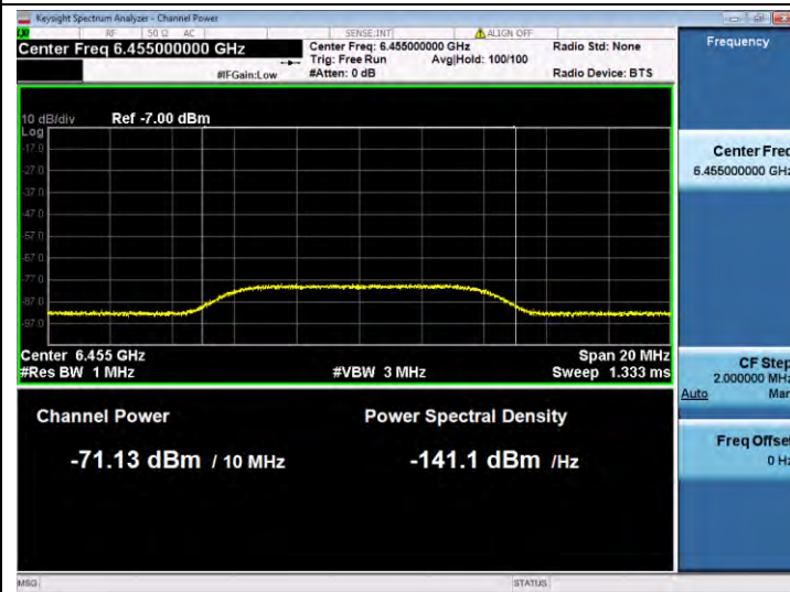
11BE20SISO-Ant 1-6455-Center-6455-Minimal
