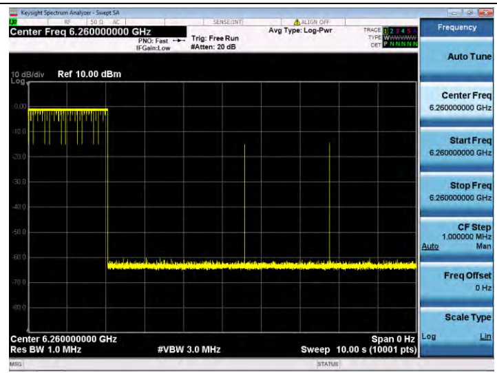
11BE320SISO-Ant 1-6260-Center-6260-Minimal
