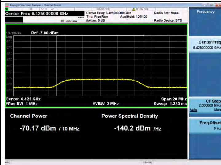
11BE320SISO-Ant 1-6425-Center-6425-Minimal
