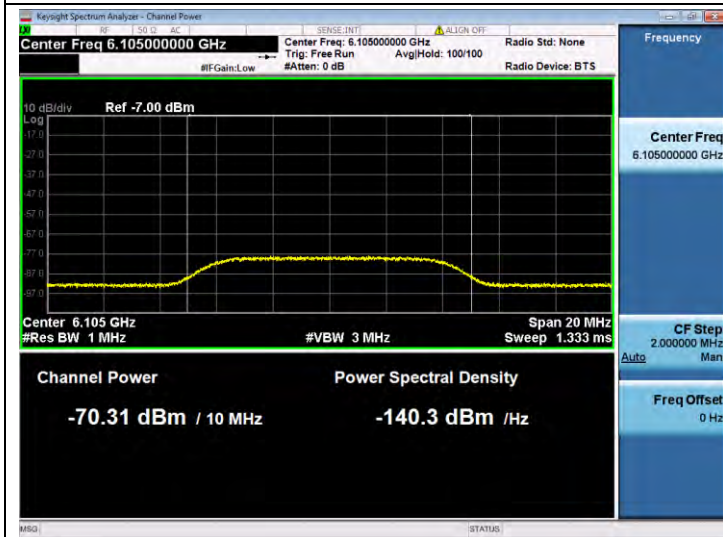
11BE320SISO-Ant 1-6105-Center-6105-Minimal
