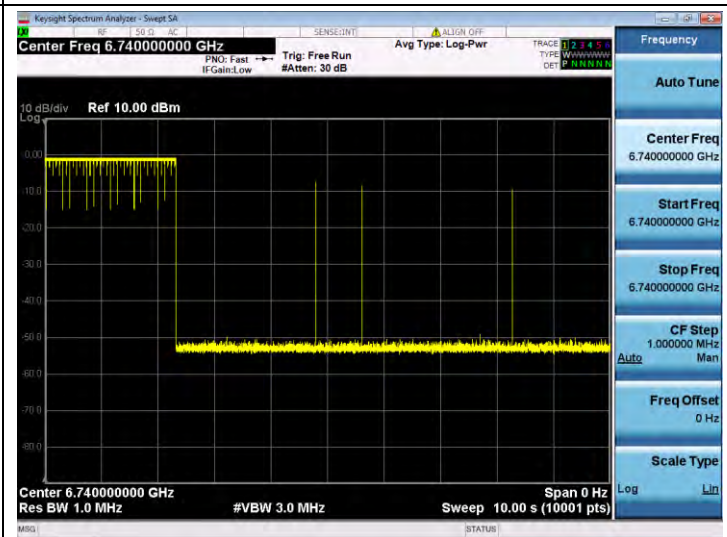
11BE320SISO-Ant 1-6585-Center-6740-Minimal
