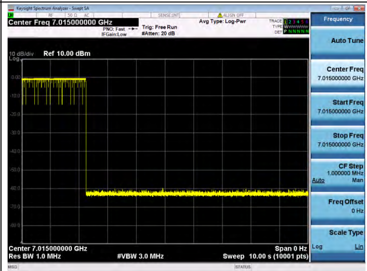
11BE20SISO-Ant 1-7015-Center-7015-Minimal
