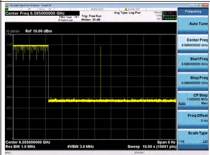
11BE320SISO-Ant 1-6585-Center-6585-Minimal
