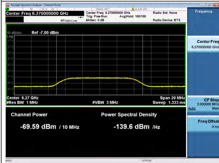
11BE320SISO-Ant 1-6425-Center-6270-Minimal
