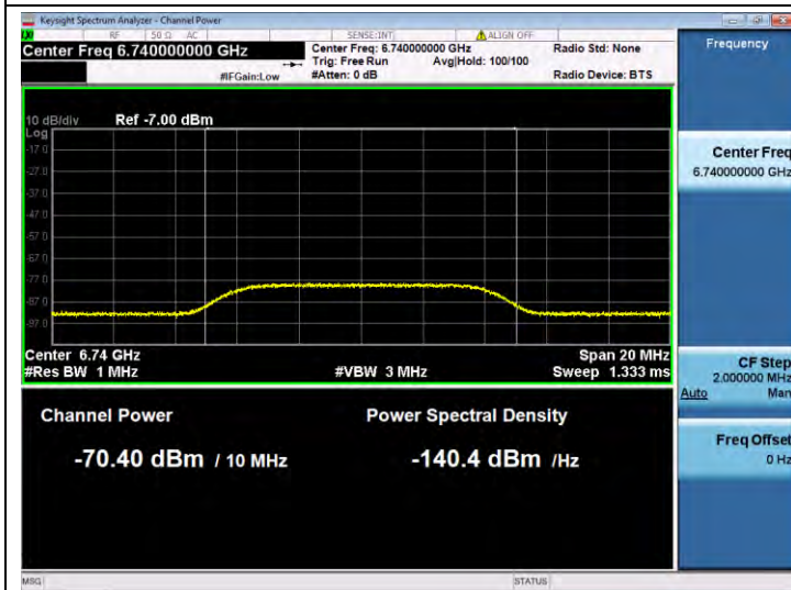
11BE320SISO-Ant 1-6585-Center-6740-Minimal
