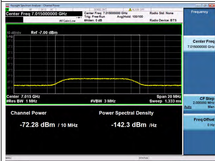
11BE20SISO-Ant 1-7015-Center-7015-Minimal
