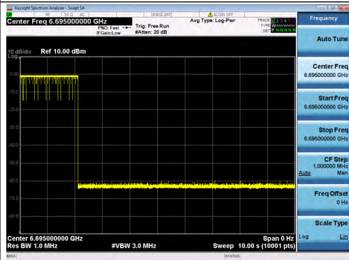
11BE20SISO-Ant 1-6695-Center-6695-Minimal
