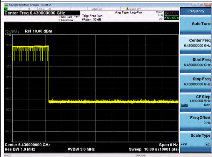
11BE320SISO-Ant 1-6585-Center-6430-Minimal
