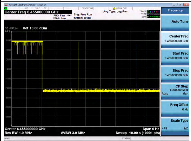
11BE20SISO-Ant 1-6455-Center-6455-Minimal
