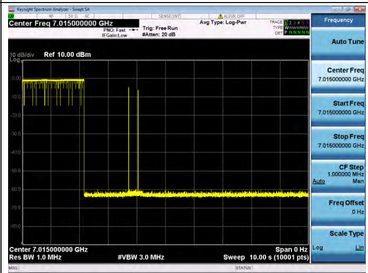
11BE20SISO-Ant 1-7015-Center-7015-Minimal
