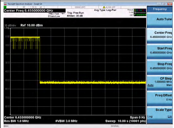
11BE20SISO-Ant 1-6455-Center-6455-Minimal
