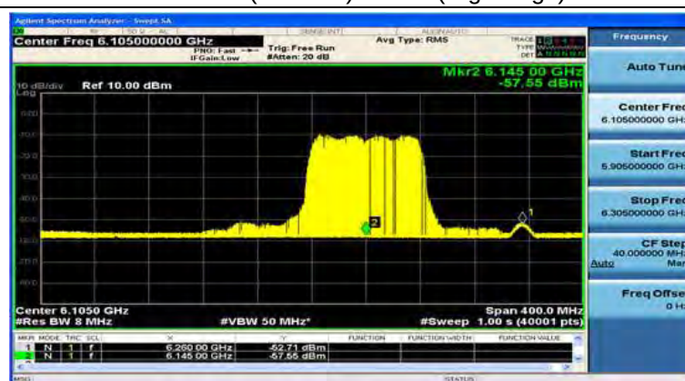
802.11be (EHT320) / CH31(High Edge)
