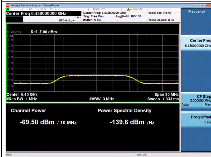
11BE320SISO-Ant 1-6585-Center-6430-Minimal
