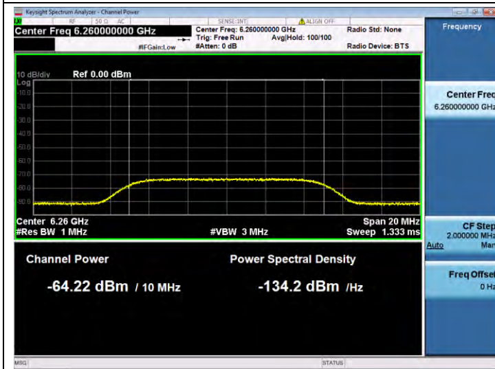
11BE320SISO-Ant 1-6260-Center-6260-Minimal
