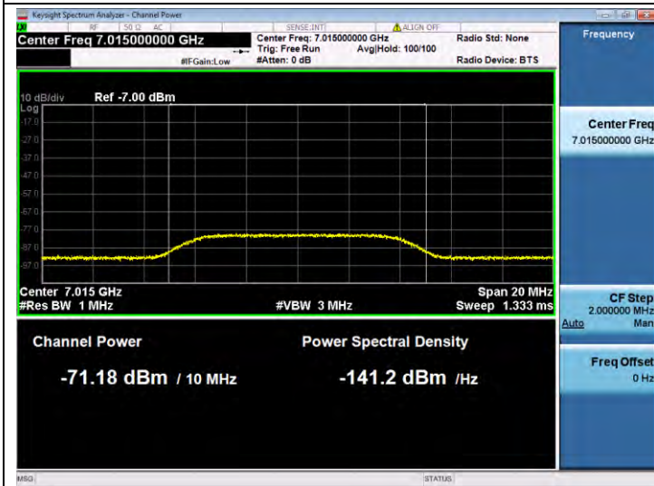
11BE20SISO-Ant 1-7015-Center-7015-Minimal
