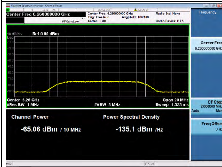
11BE320SISO-Ant 1-6260-Center-6260-Minimal
