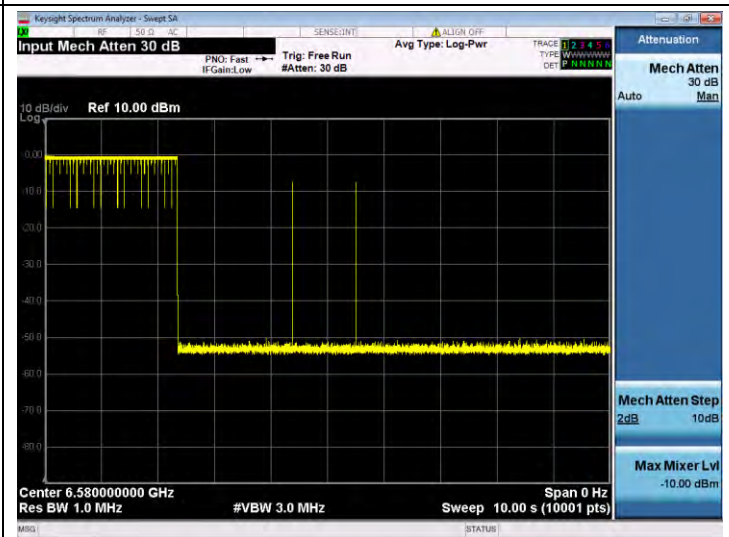
11BE320SISO-Ant 1-6425-Center-6580-Minimal
