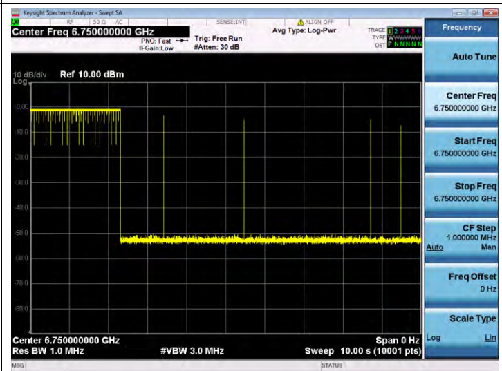
11BE320SISO-Ant 1-6905-Center-6750-Minimal
