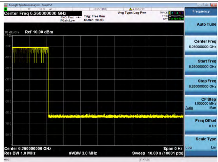
11BE320SISO-Ant 1-6260-Center-6260-Minimal
