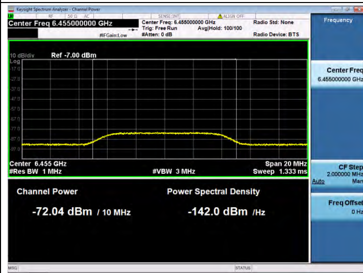
11BE20SISO-Ant 1-6455-Center-6455-Minimal
