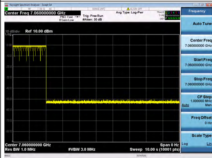
11BE320SISO-Ant 1-6905-Center-7060-Minimal
