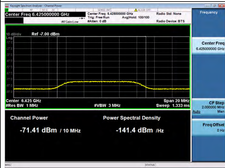
11BE320SISO-Ant 1-6425-Center-6425-Minimal
