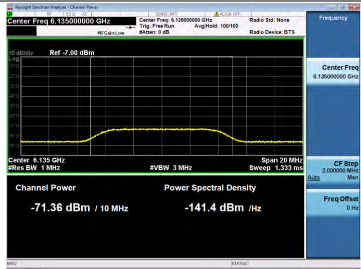
11BE20SISO-Ant 1-6135-Center-6135-Minimal
