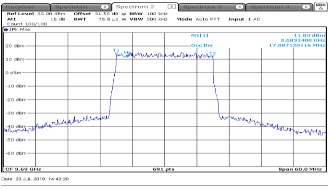
Figure 8.3-2: Occupied bandwidth sample plot for 1CC 20 MHz channel
