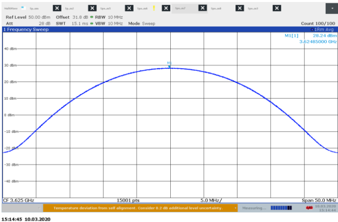
Figure 8.1-1: Ouput power sample plot, 1cc 10 MHz channel
