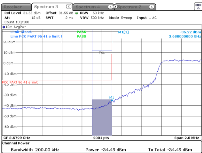
Figure 8.4-6: Emission measurement within 0-1 MHz low end from the SAS assigned channel edge, sample plot for 2CC 10 MHz channel
