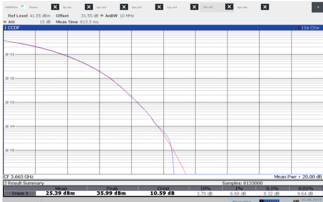
Figure 8.2-6: CCDF sample plot, 3cc 20 MHz channel
