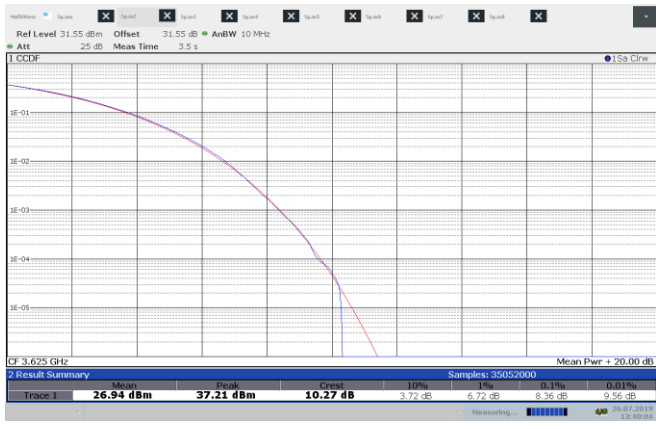
Figure 8.2-2: CCDF sample plot, 1cc 20 MHz channel
