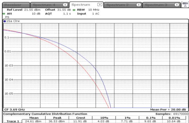
Figure 8.2-3: CCDF sample plot, 2cc 10 MHz channel
