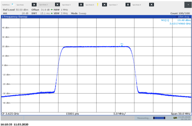
Figure 8.1-4: Power spectral density sample plot 1cc, 20 MHz channel
