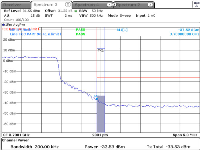
Figure 8.4-15: Emission measurement within 0-1 MHz high end from the SAS assigned channel edge, sample plot for 1CC 20 MHz channel
