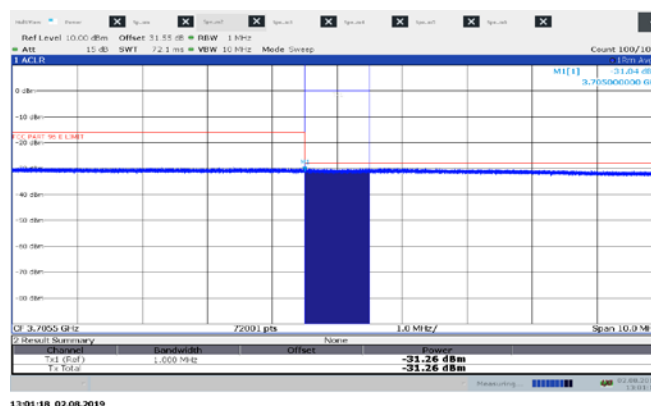
Figure 8.4-28: Band edge measurement outside 10 MHz high end from the SAS assigned channel edge, sample plot for 3CC 20 MHz channel
