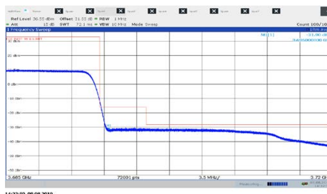
Figure 8.4-26: Emission measurement within 1-10 MHz and outside 10 MHz high end from the SAS assigned channel edge, sample plot for 3CC 20 MHz channel
