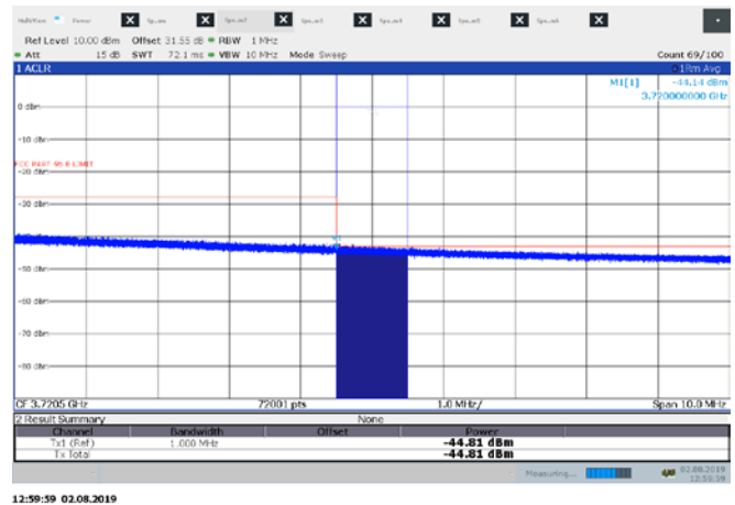
Figure 8.5-19: Emission measurement at 3720 MHz for 3CC 20 MHz sample plot
