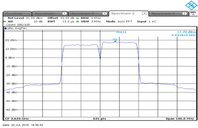
Figure 8.1-8: Power spectral density sample plot, 20 MHz channel
