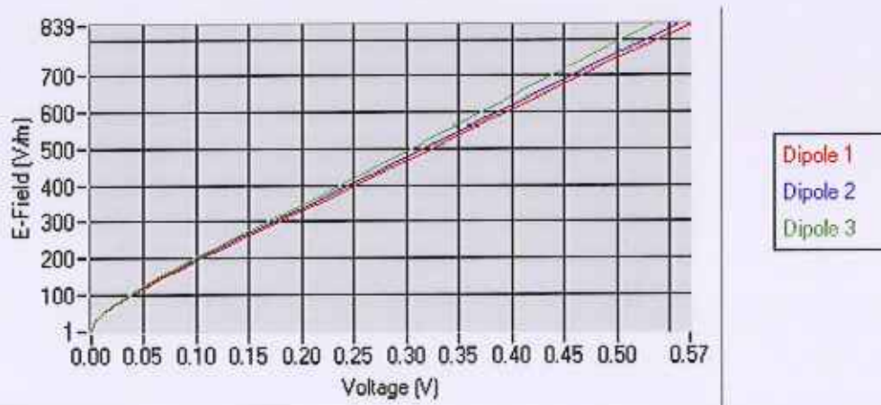
Calibration curves
