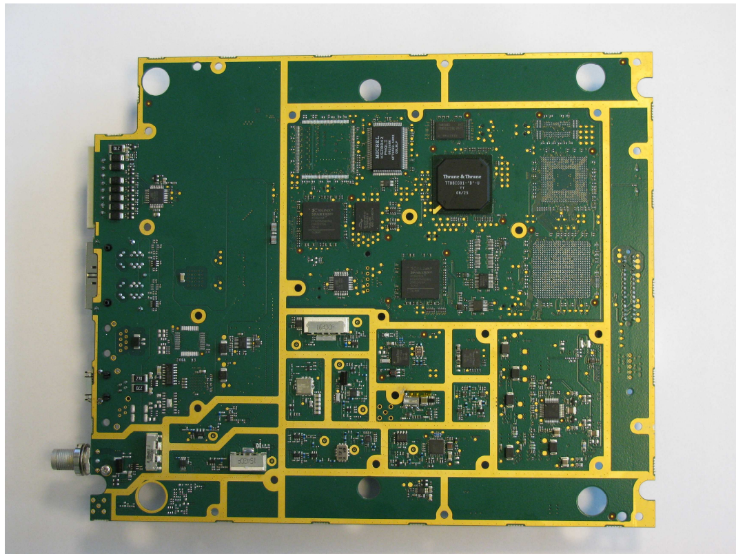
Figur 4 MainBoard
