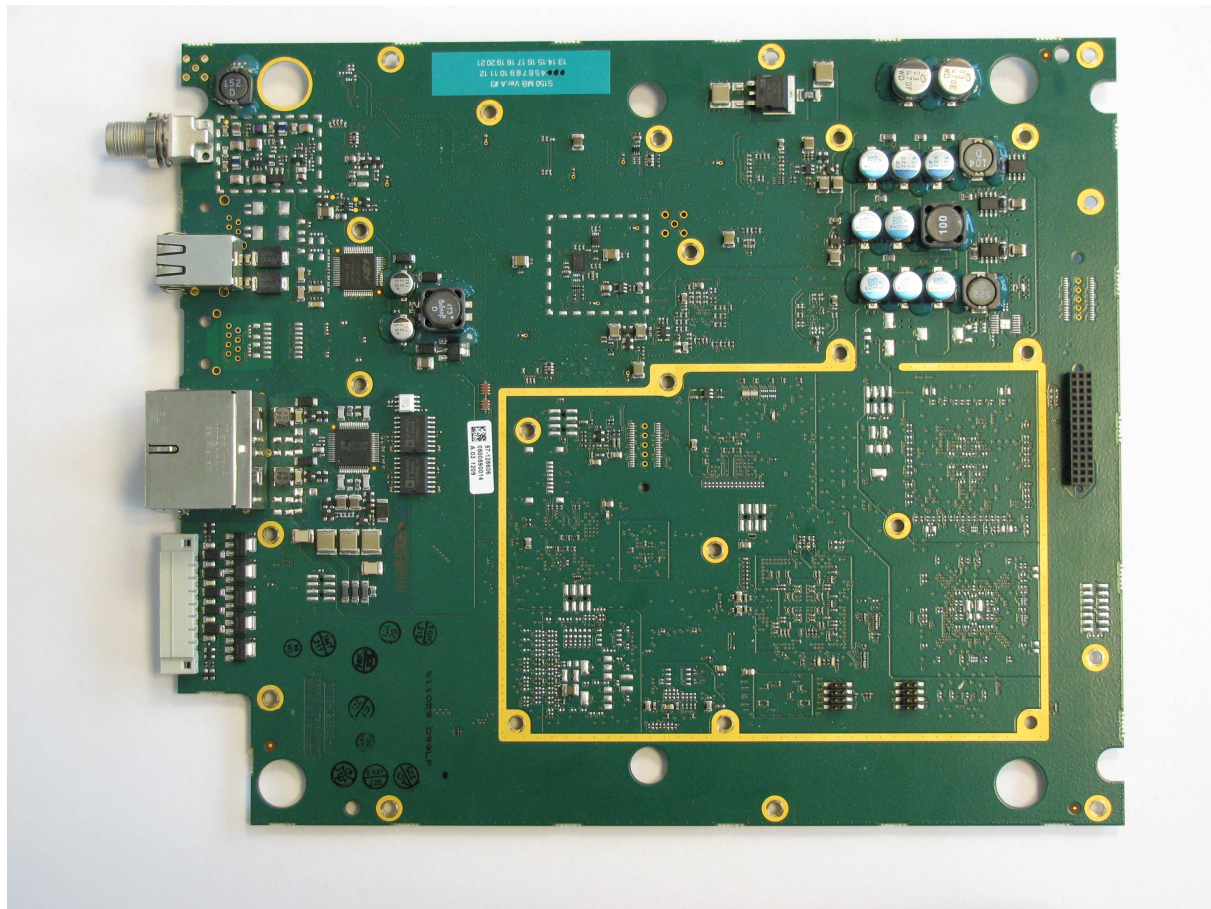
Figur 3 MainBoard
