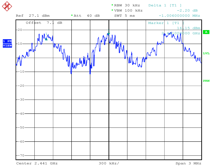
Figure 2. Channel separation
