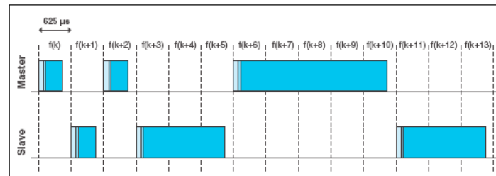
Figure 2.1: Multi-slot packets
