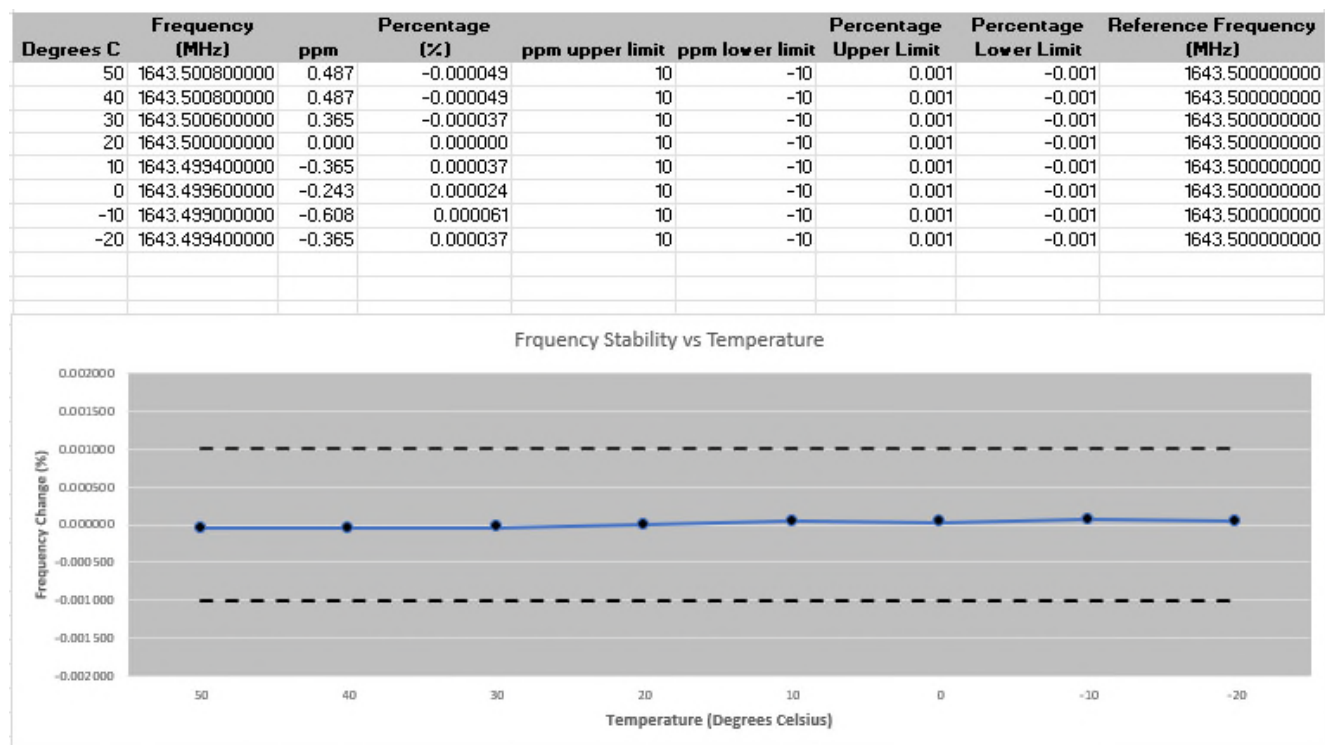
Figure 2.6.6-3: Frequency Stability at Various Temperatures – Mid Channel
