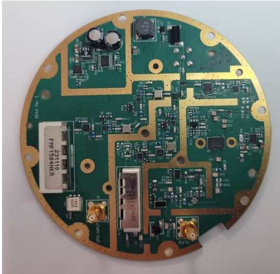
Yahsat T-TAC Vehicular Antenna PCBA TopView
