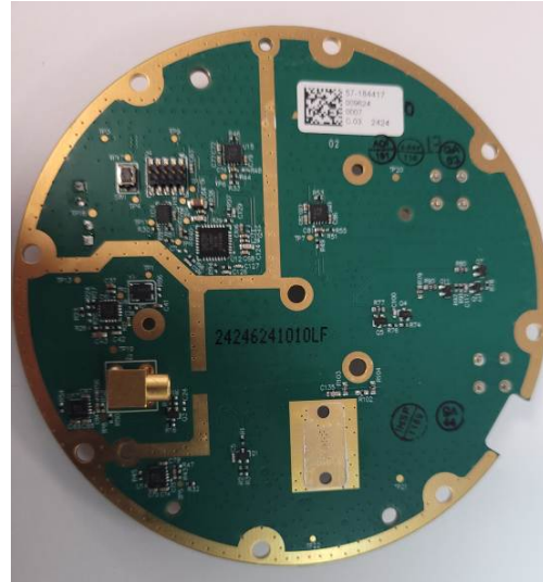
Yahsat T-TAC Vehicular Antenna PCBA BottomView
