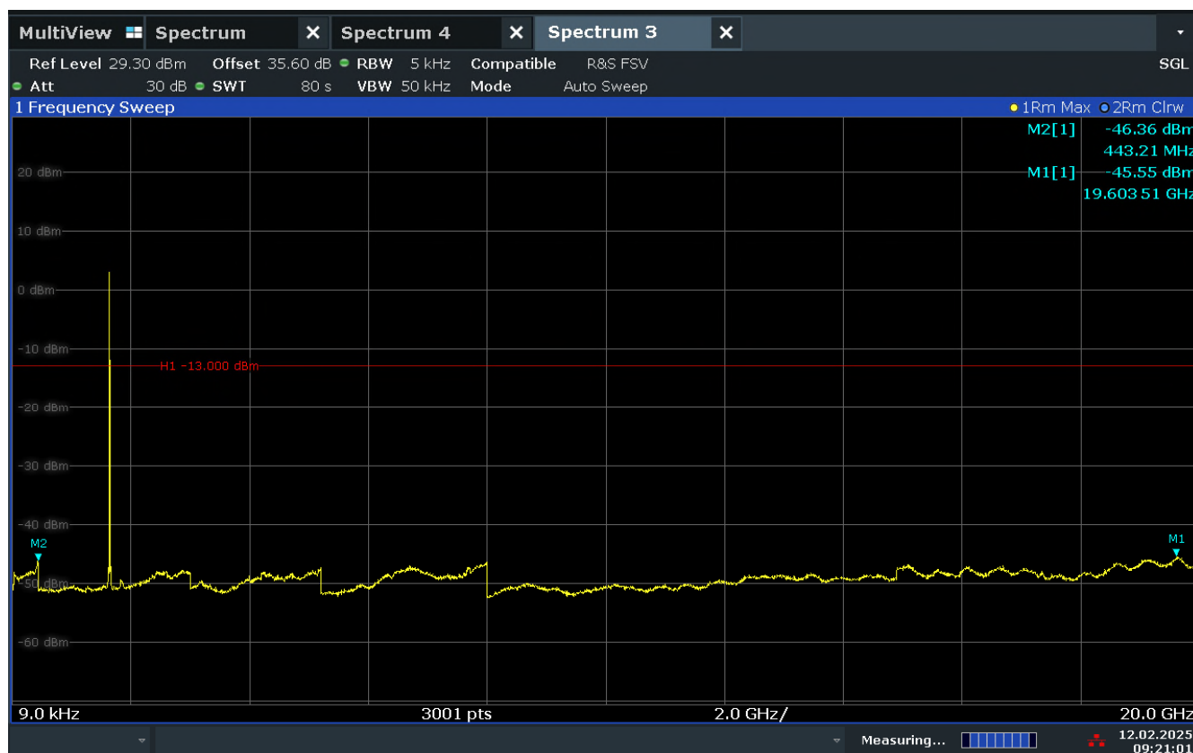
Figure 2-10 – Conducted Spurious Emissions 9 kHz – 20GHz – Mid Channel
