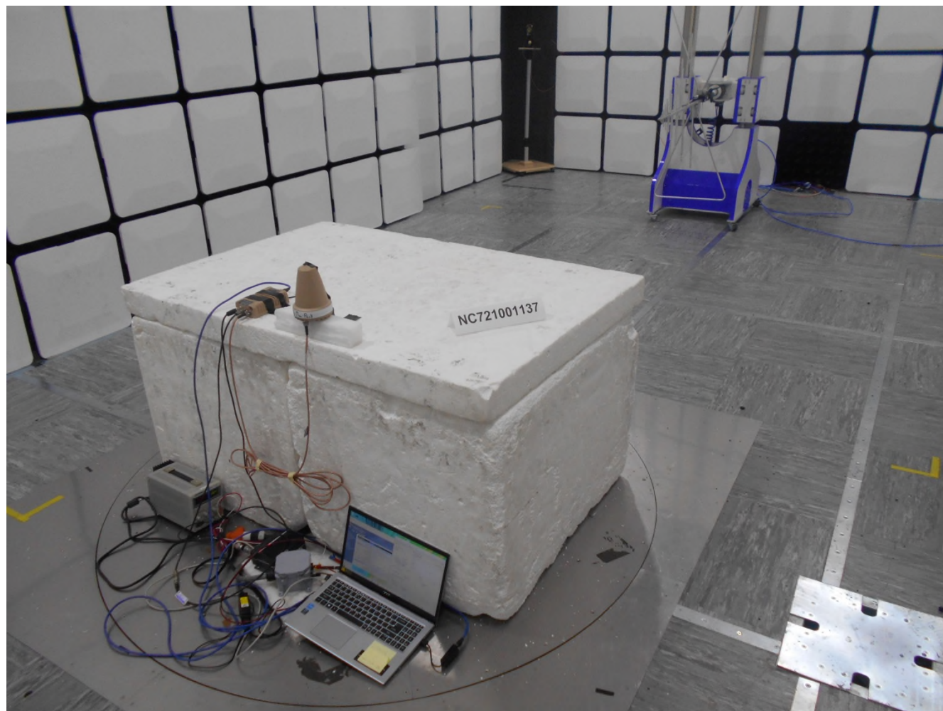
Photo 1.3-1 – RE Spurious Emissions 30-1000 MHz
