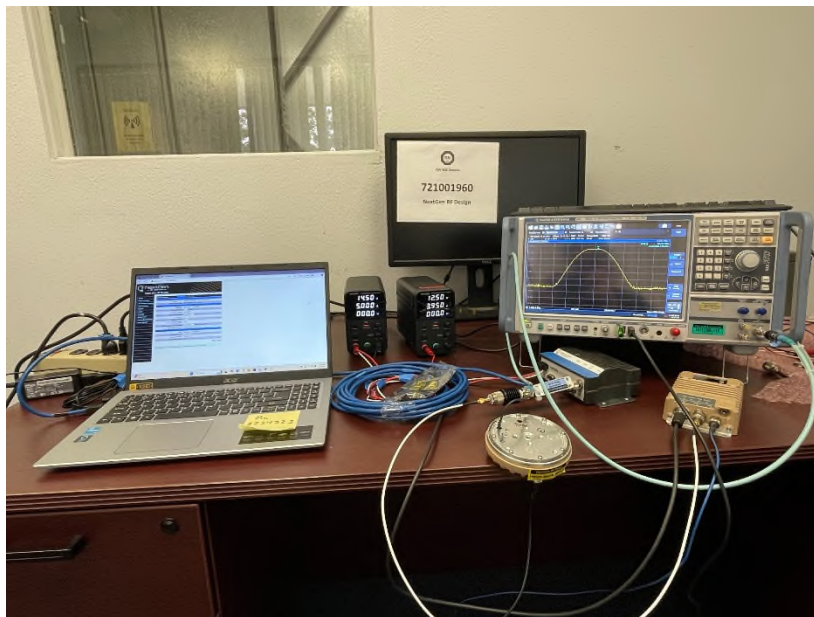
Photo 1.1-1 – Conducted Test Setup
