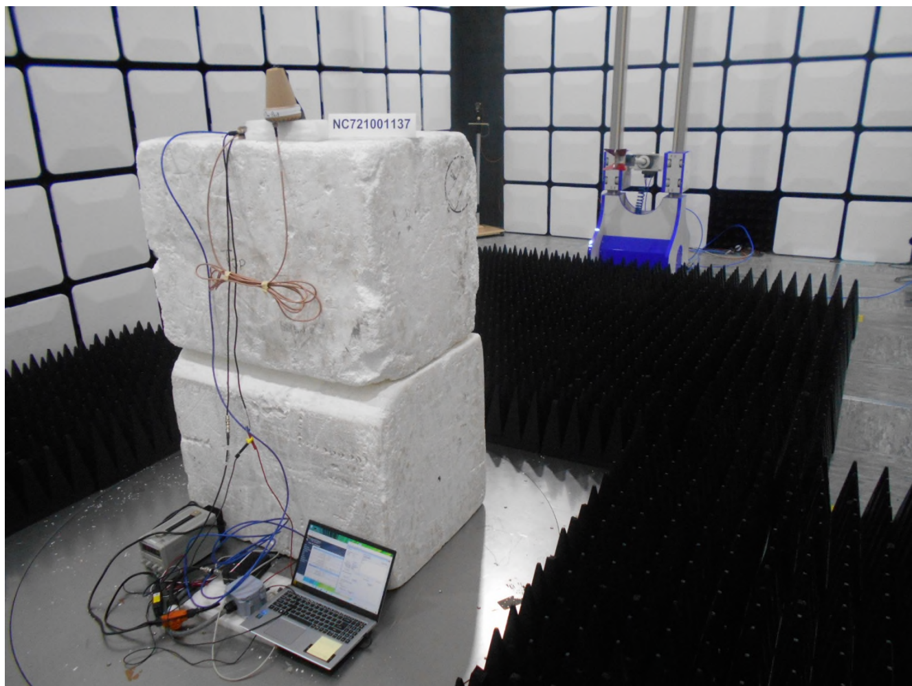
Photo 1.3-2 – RE Spurious Emissions 1-18 GHz
