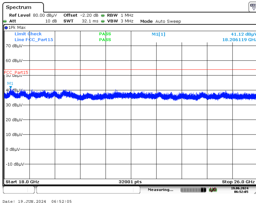
Plot 2: Lowest channel, 18 GHz to 26 GHz, vertical & horizontal polarization
