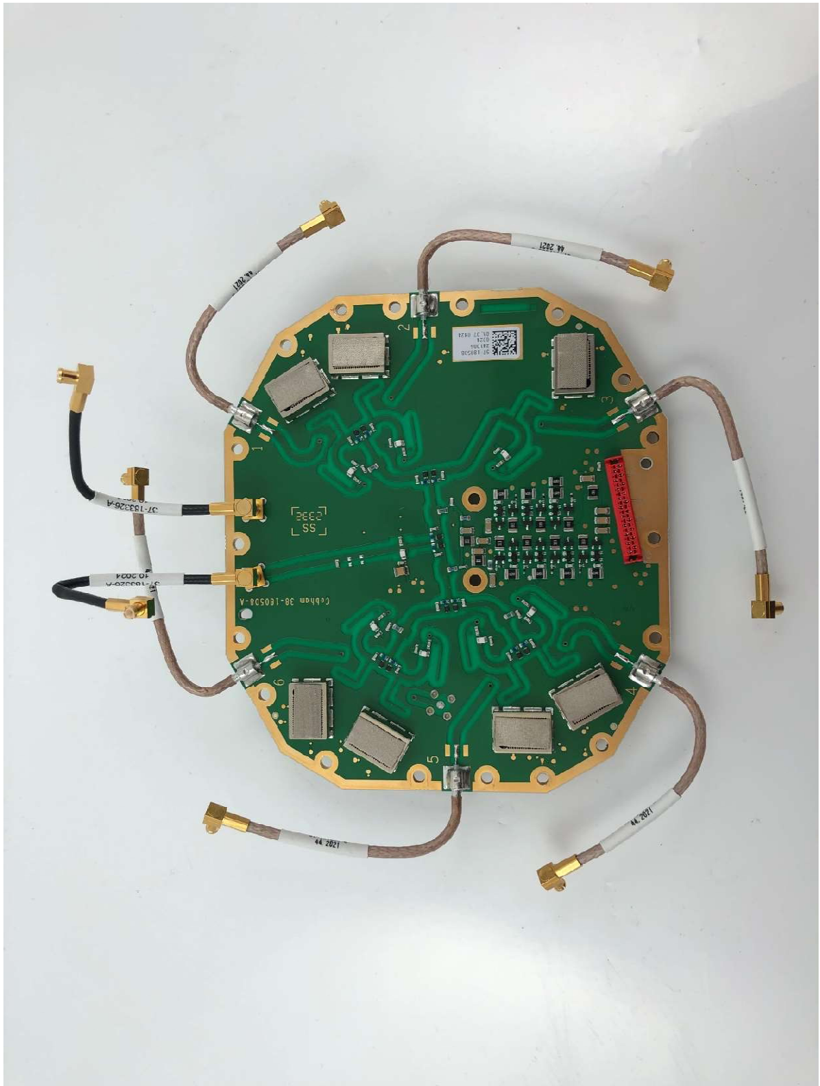
Switch Board
